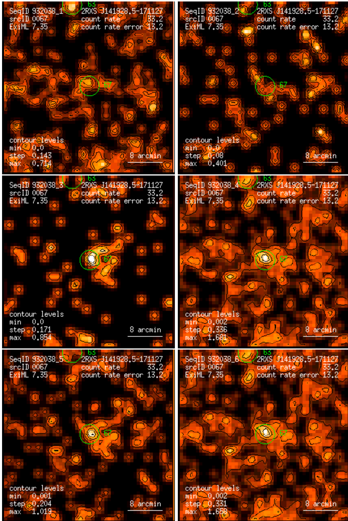
Figure 67: RASS 932038: detection 0067: band rate images, Gaussian filter: (1) PSPC channels 11 – 41, (2) 52 – 90, (3) 91 – 201, (4) 11 – 235, (5) 52 – 201, (6) 11 – 201. Broad band rates in counts/ks. Band rate contour levels in counts/ks/arcmin 2 .
