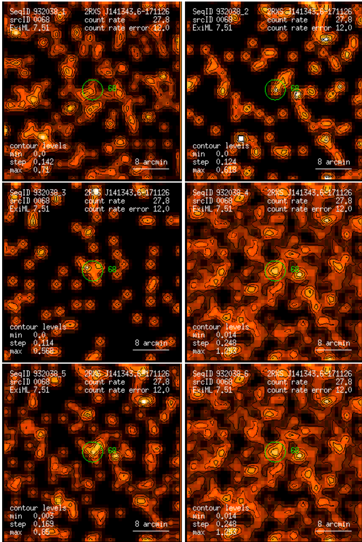
Figure 68: RASS 932038: detection 0068: band rate images, Gaussian filter: (1) PSPC channels 11 – 41, (2) 52 – 90, (3) 91 – 201, (4) 11 – 235, (5) 52 – 201, (6) 11 – 201. Broad band rates in counts/ks. Band rate contour levels in counts/ks/arcmin 2 .
