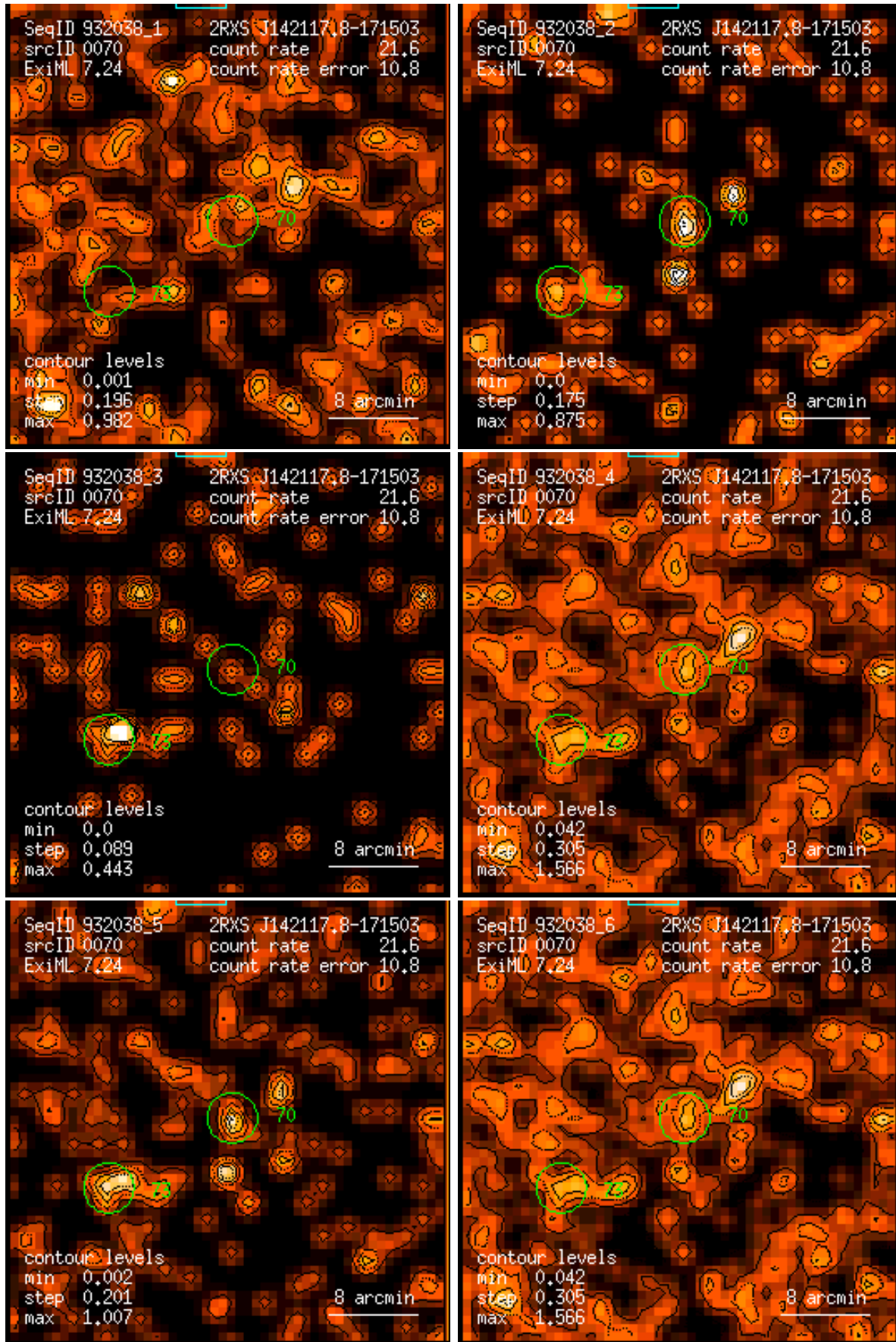
Figure 70: RASS 932038: detection 0070: band rate images, Gaussian filter: (1) PSPC channels 11 – 41, (2) 52 – 90, (3) 91 – 201, (4) 11 – 235, (5) 52 – 201, (6) 11 – 201. Broad band rates in counts/ks. Band rate contour levels in counts/ks/arcmin 2 .
