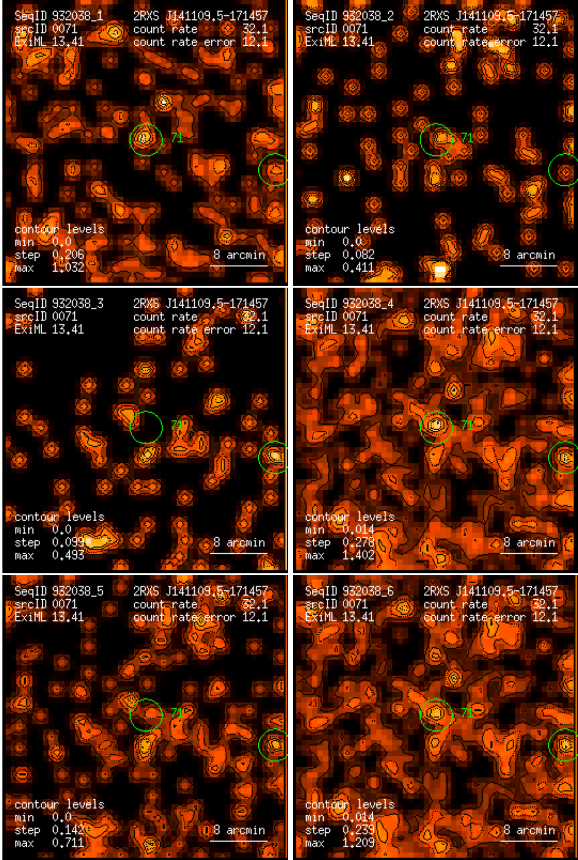
Figure 71: RASS 932038: detection 0071: band rate images, Gaussian filter: (1) PSPC channels 11 – 41, (2) 52 – 90, (3) 91 – 201, (4) 11 – 235, (5) 52 – 201, (6) 11 – 201. Broad band rates in counts/ks. Band rate contour levels in counts/ks/arcmin 2 .
