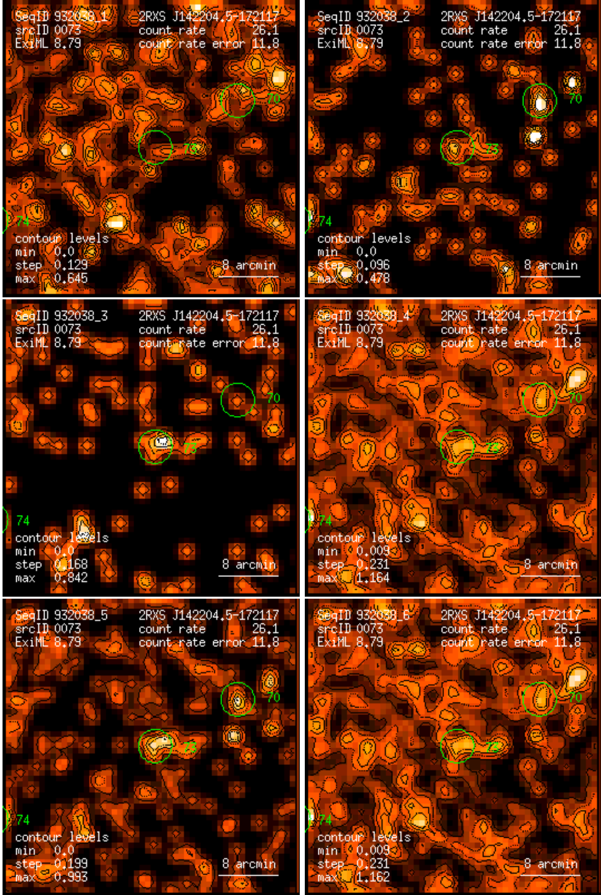
Figure 73: RASS 932038: detection 0073: band rate images, Gaussian filter: (1) PSPC channels 11 – 41, (2) 52 – 90, (3) 91 – 201, (4) 11 – 235, (5) 52 – 201, (6) 11 – 201. Broad band rates in counts/ks. Band rate contour levels in counts/ks/arcmin 2 .
