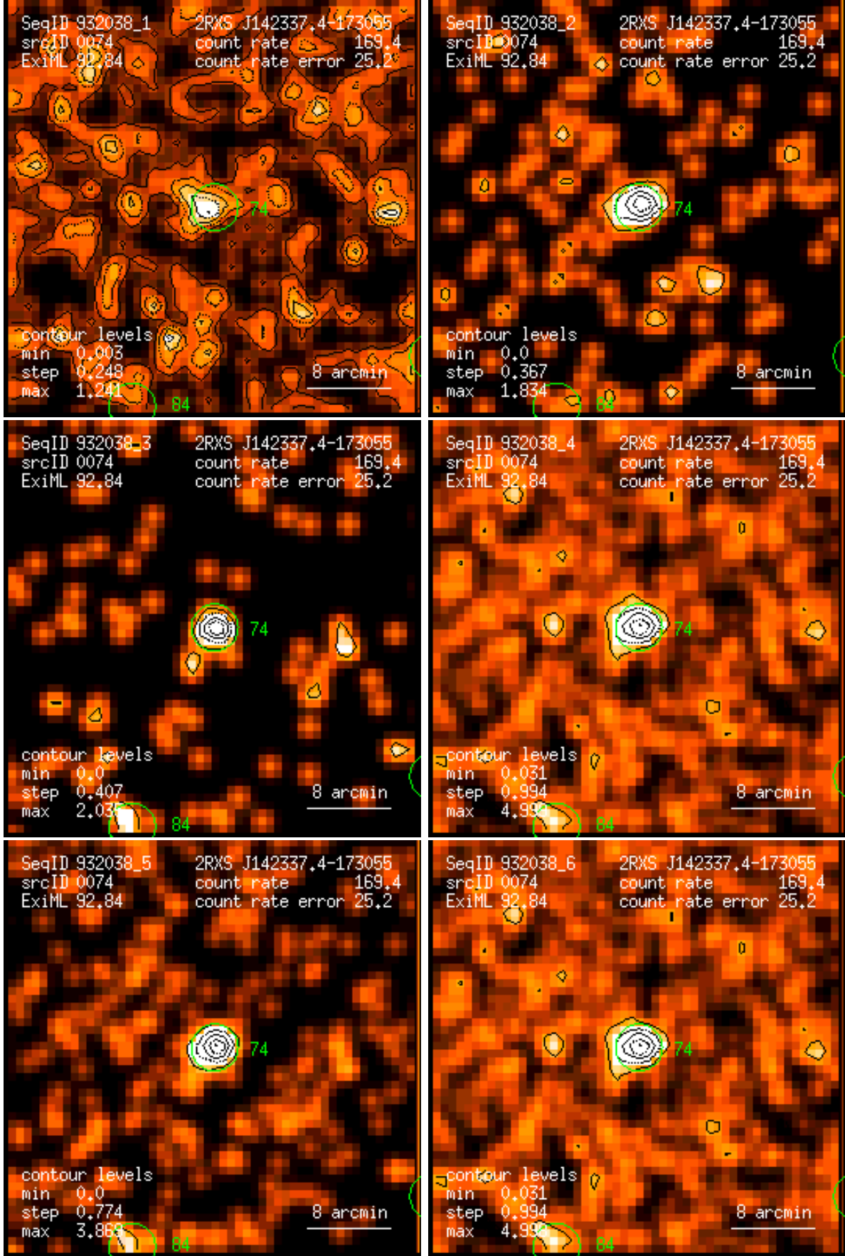
Figure 74: RASS 932038: detection 0074: band rate images, Gaussian filter: (1) PSPC channels 11 – 41, (2) 52 – 90, (3) 91 – 201, (4) 11 – 235, (5) 52 – 201, (6) 11 – 201. Broad band rates in counts/ks. Band rate contour levels in counts/ks/arcmin 2 .
