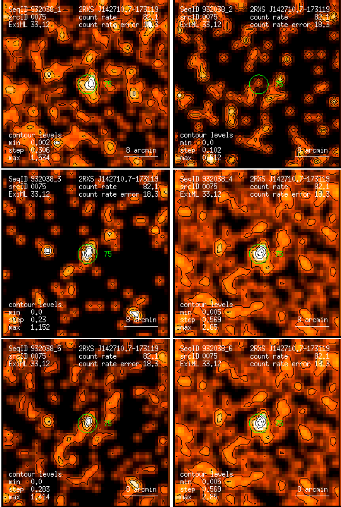
Figure 75: RASS 932038: detection 0075: band rate images, Gaussian filter: (1) PSPC channels 11 – 41, (2) 52 – 90, (3) 91 – 201, (4) 11 – 235, (5) 52 – 201, (6) 11 – 201. Broad band rates in counts/ks. Band rate contour levels in counts/ks/arcmin 2 .
