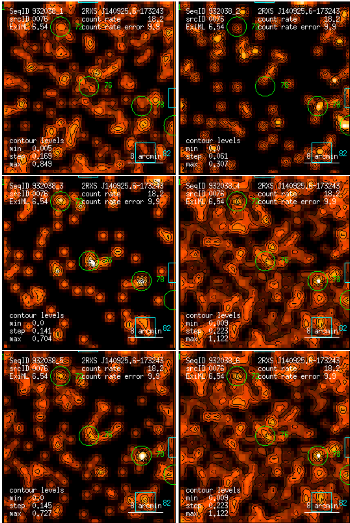
Figure 76: RASS 932038: detection 0076: band rate images, Gaussian filter: (1) PSPC channels 11 – 41, (2) 52 – 90, (3) 91 – 201, (4) 11 – 235, (5) 52 – 201, (6) 11 – 201. Broad band rates in counts/ks. Band rate contour levels in counts/ks/arcmin 2 .
