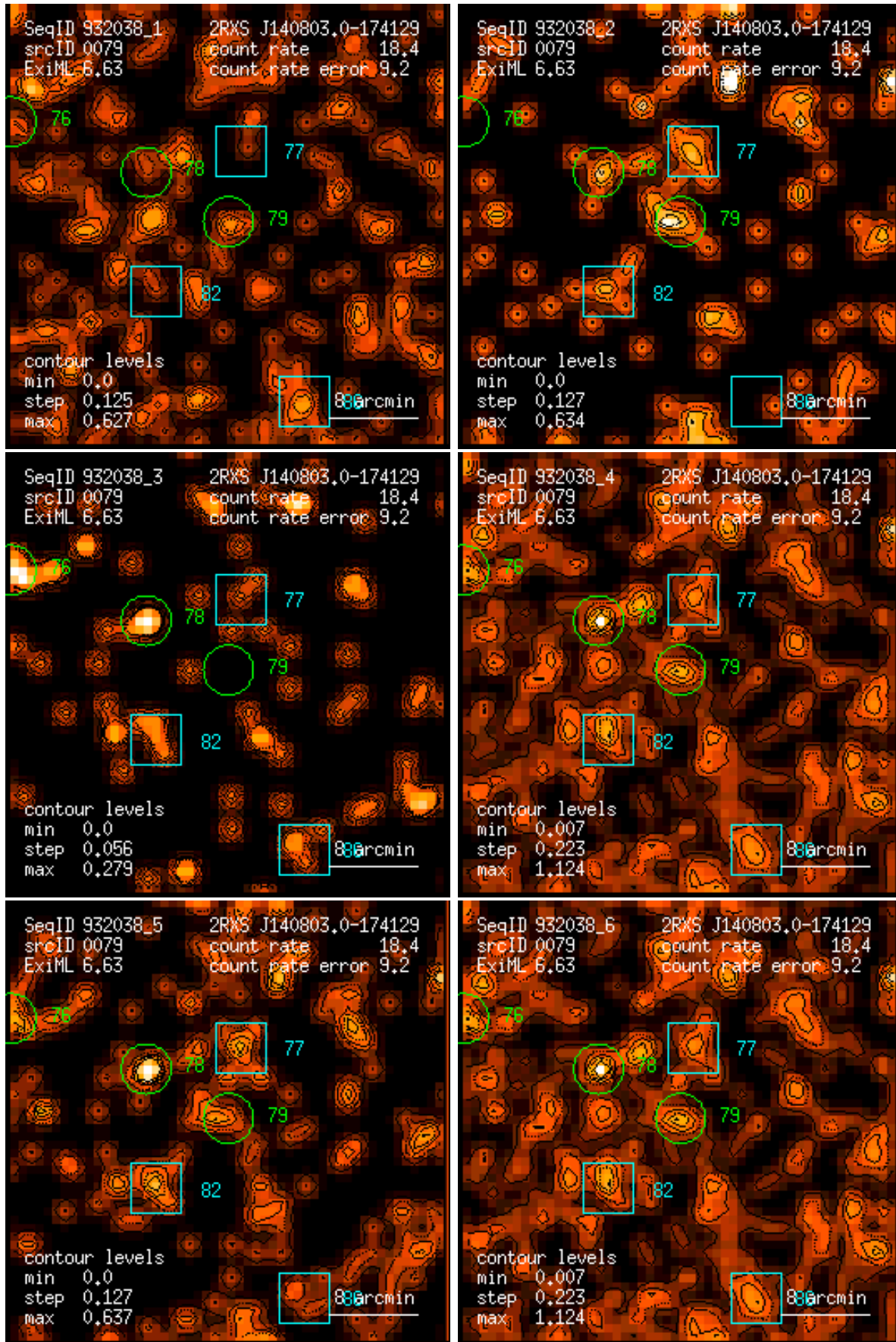
Figure 79: RASS 932038: detection 0079: band rate images, Gaussian filter: (1) PSPC channels 11 – 41, (2) 52 – 90, (3) 91 – 201, (4) 11 – 235, (5) 52 – 201, (6) 11 – 201. Broad band rates in counts/ks. Band rate contour levels in counts/ks/arcmin 2 .
