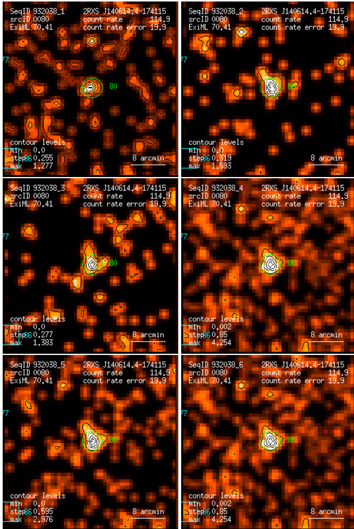
Figure 80: RASS 932038: detection 0080: band rate images, Gaussian filter: (1) PSPC channels 11 – 41, (2) 52 – 90, (3) 91 – 201, (4) 11 – 235, (5) 52 – 201, (6) 11 – 201. Broad band rates in counts/ks. Band rate contour levels in counts/ks/arcmin 2 .
