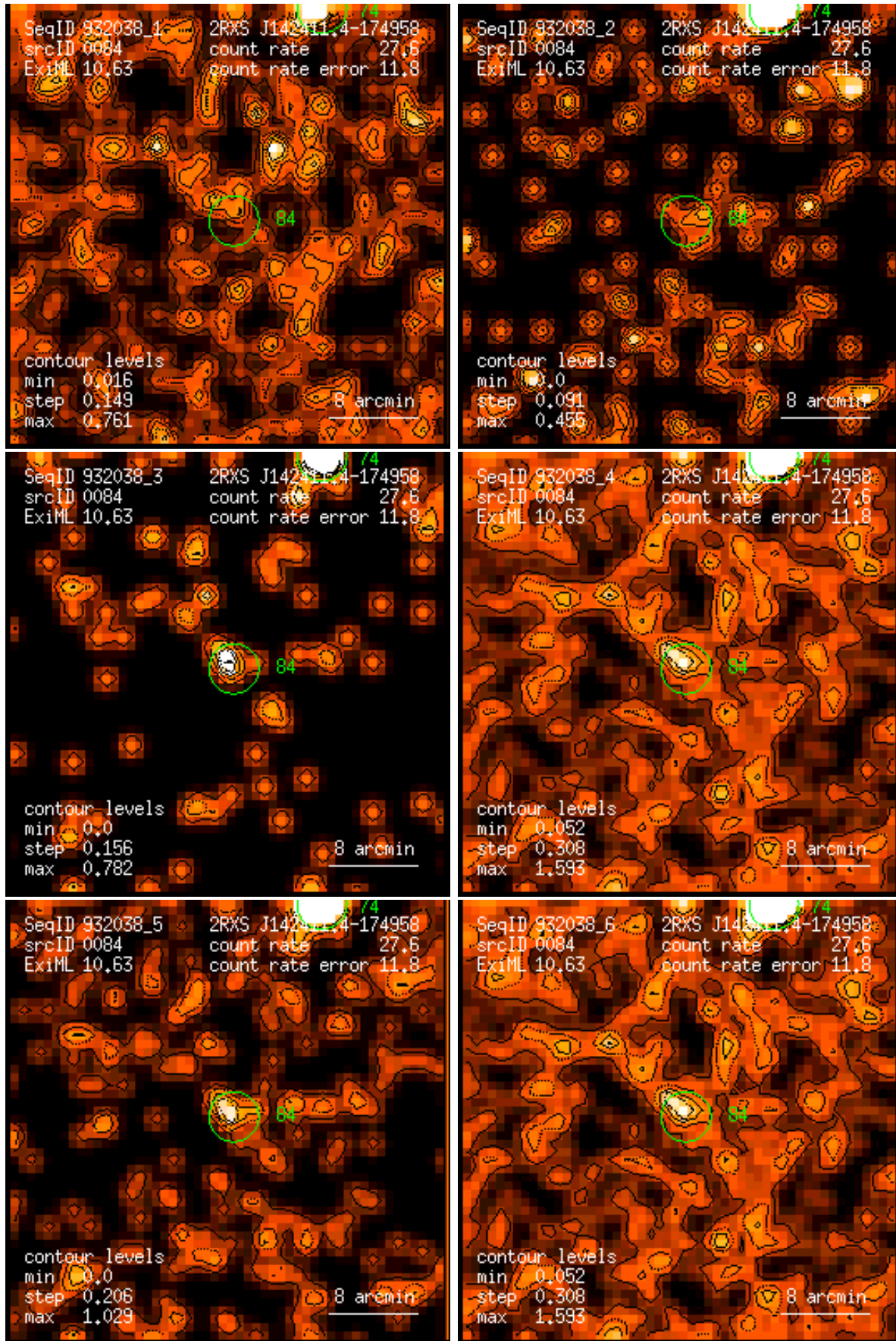
Figure 84: RASS 932038: detection 0084: band rate images, Gaussian filter: (1) PSPC channels 11 – 41, (2) 52 – 90, (3) 91 – 201, (4) 11 – 235, (5) 52 – 201, (6) 11 – 201. Broad band rates in counts/ks. Band rate contour levels in counts/ks/arcmin 2 .
