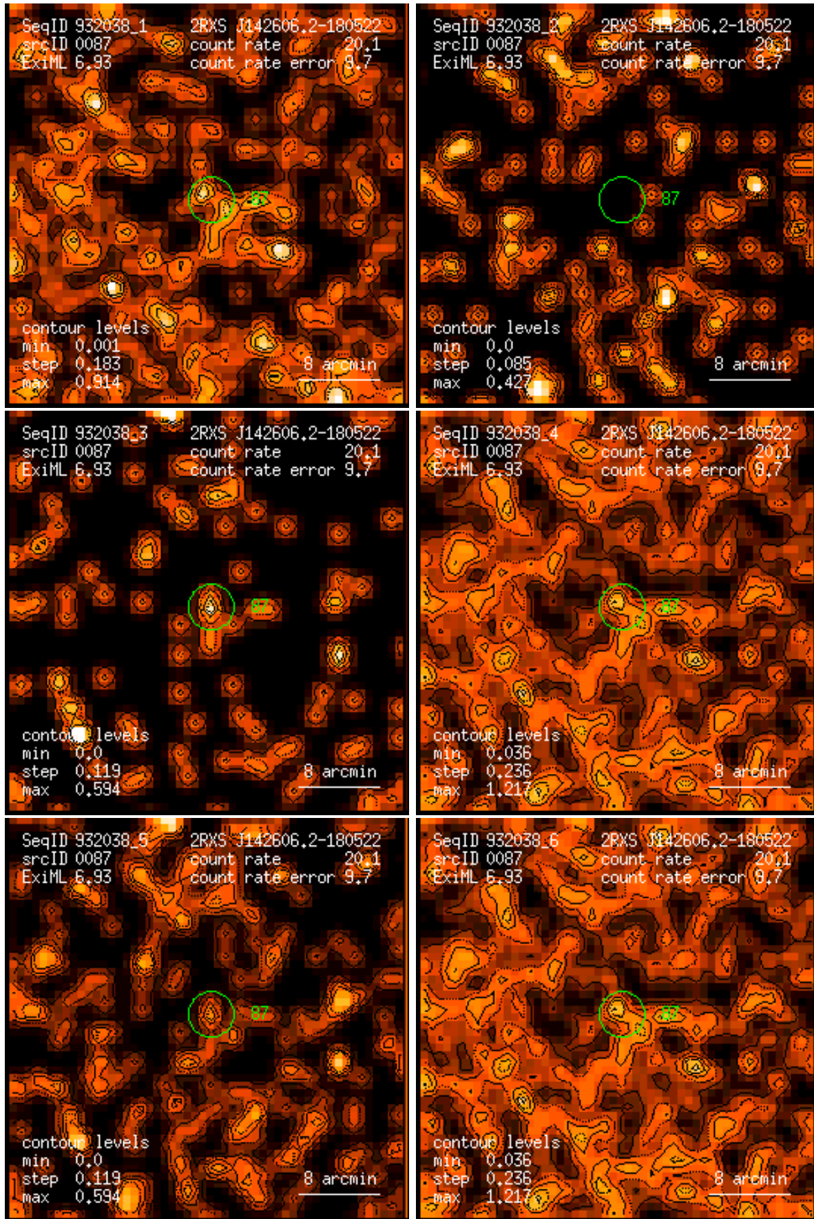
Figure 87: RASS 932038: detection 0087: band rate images, Gaussian filter: (1) PSPC channels 11 – 41, (2) 52 – 90, (3) 91 – 201, (4) 11 – 235, (5) 52 – 201, (6) 11 – 201. Broad band rates in counts/ks. Band rate contour levels in counts/ks/arcmin 2 .
