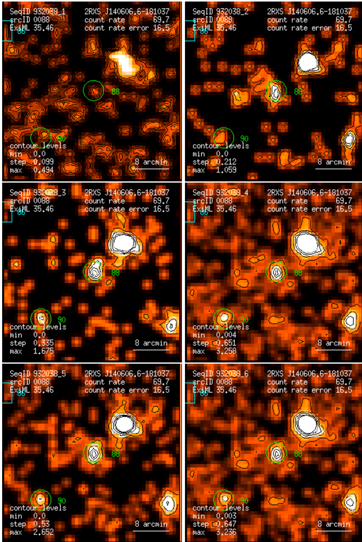
Figure 88: RASS 932038: detection 0088: band rate images, Gaussian filter: (1) PSPC channels 11 – 41, (2) 52 – 90, (3) 91 – 201, (4) 11 – 235, (5) 52 – 201, (6) 11 – 201. Broad band rates in counts/ks. Band rate contour levels in counts/ks/arcmin 2 .
