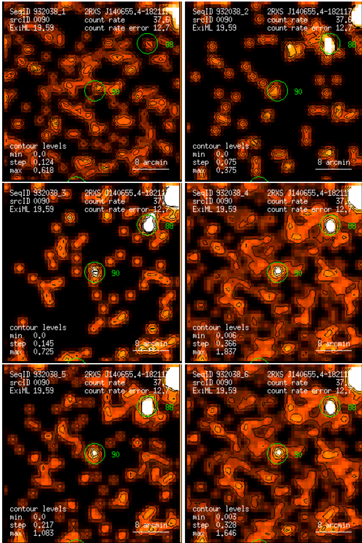
Figure 90: RASS 932038: detection 0090: band rate images, Gaussian filter: (1) PSPC channels 11 – 41, (2) 52 – 90, (3) 91 – 201, (4) 11 – 235, (5) 52 – 201, (6) 11 – 201. Broad band rates in counts/ks. Band rate contour levels in counts/ks/arcmin 2 .
