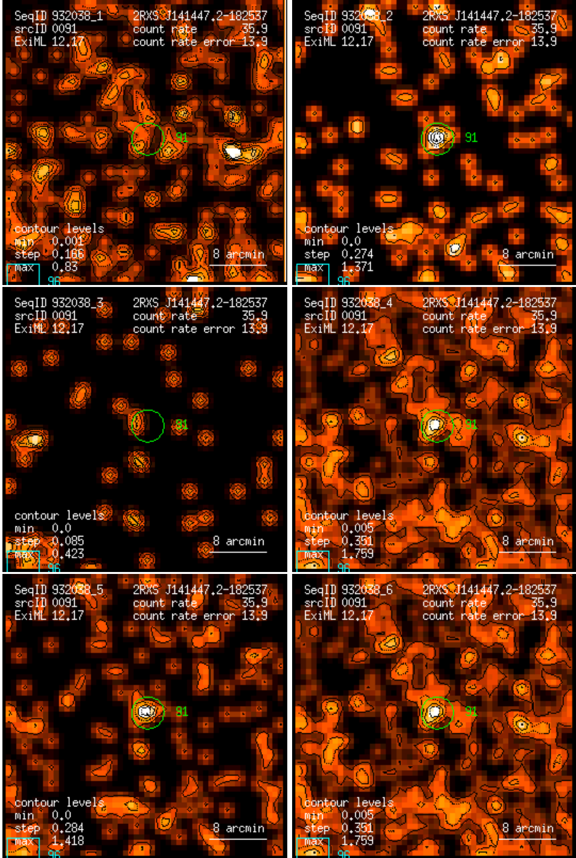
Figure 91: RASS 932038: detection 0091: band rate images, Gaussian filter: (1) PSPC channels 11 – 41, (2) 52 – 90, (3) 91 – 201, (4) 11 – 235, (5) 52 – 201, (6) 11 – 201. Broad band rates in counts/ks. Band rate contour levels in counts/ks/arcmin 2 .
