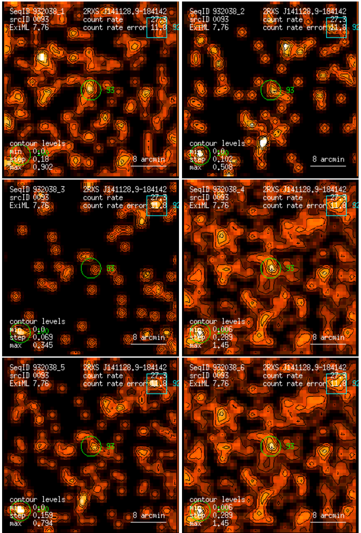
Figure 93: RASS 932038: detection 0093: band rate images, Gaussian filter: (1) PSPC channels 11 – 41, (2) 52 – 90, (3) 91 – 201, (4) 11 – 235, (5) 52 – 201, (6) 11 – 201. Broad band rates in counts/ks. Band rate contour levels in counts/ks/arcmin 2 .
