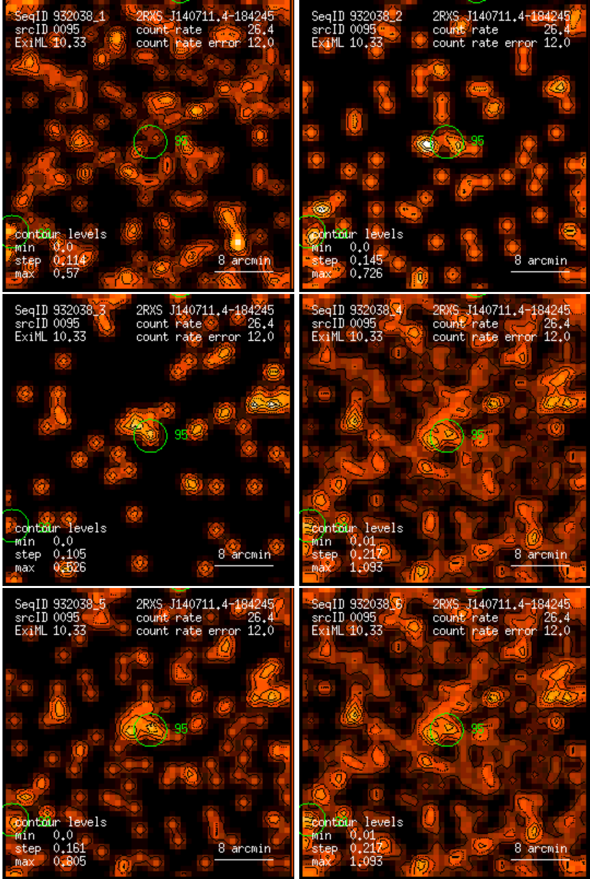
Figure 95: RASS 932038: detection 0095: band rate images, Gaussian filter: (1) PSPC channels 11 – 41, (2) 52 – 90, (3) 91 – 201, (4) 11 – 235, (5) 52 – 201, (6) 11 – 201. Broad band rates in counts/ks. Band rate contour levels in counts/ks/arcmin 2 .
