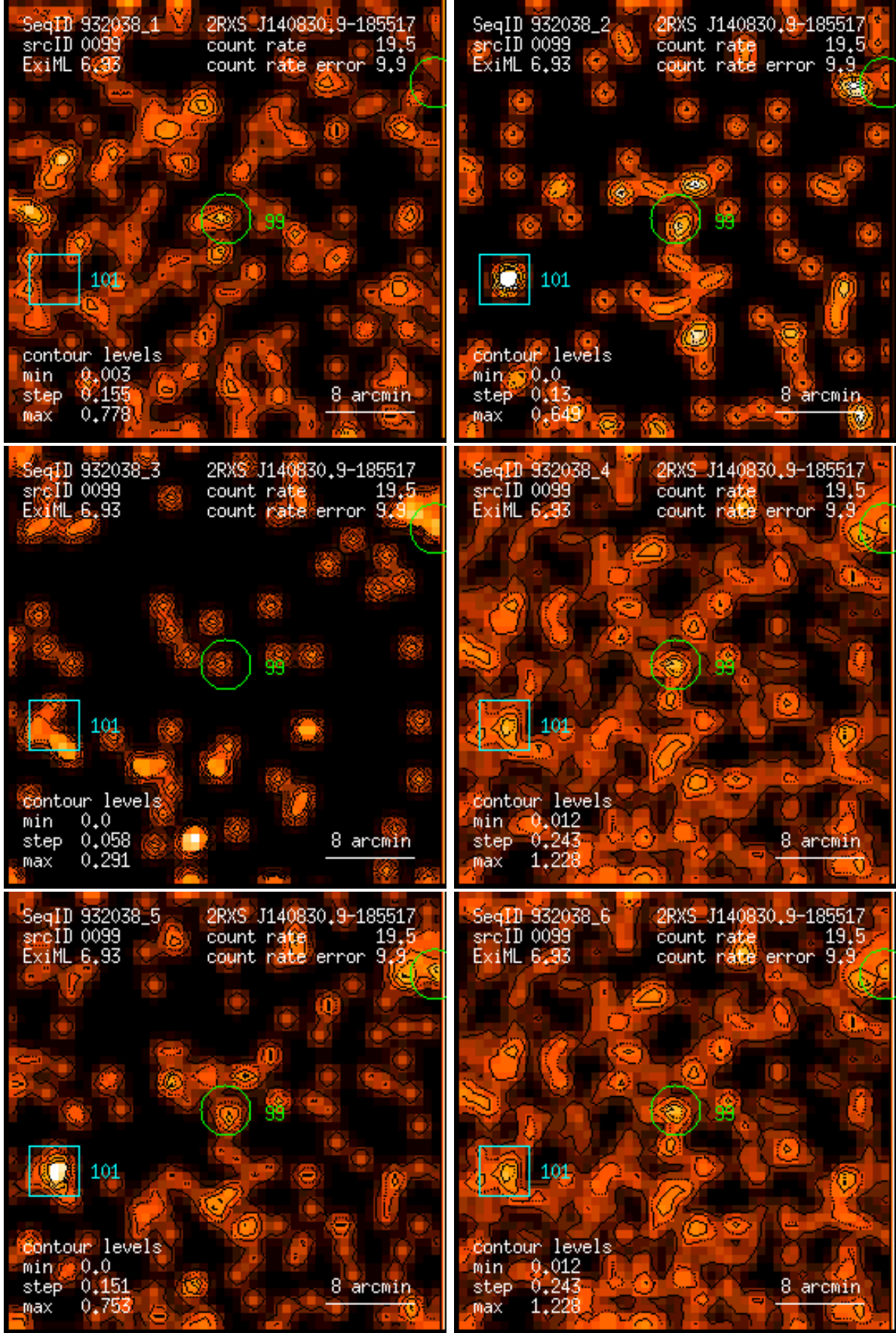
Figure 99: RASS 932038: detection 0099: band rate images, Gaussian filter: (1) PSPC channels 11 – 41, (2) 52 – 90, (3) 91 – 201, (4) 11 – 235, (5) 52 – 201, (6) 11 – 201. Broad band rates in counts/ks. Band rate contour levels in counts/ks/arcmin 2 .
