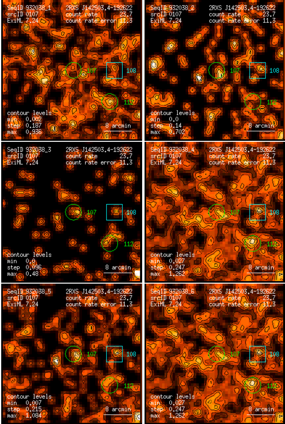
Figure 107: RASS 932038: detection 0107: band rate images, Gaussian filter: (1) PSPC channels 11 – 41, (2) 52 – 90, (3) 91 – 201, (4) 11 – 235, (5) 52 – 201, (6) 11 – 201. Broad band rates in counts/ks. Band rate contour levels in counts/ks/arcmin 2 .
