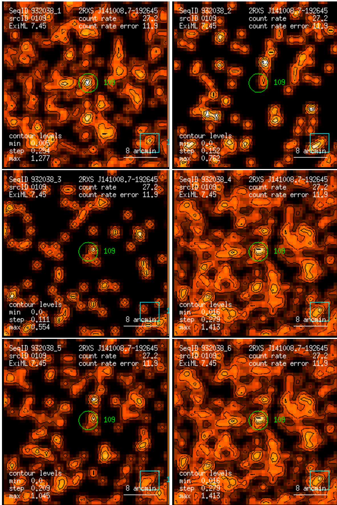
Figure 109: RASS 932038: detection 0109: band rate images, Gaussian filter: (1) PSPC channels 11 – 41, (2) 52 – 90, (3) 91 – 201, (4) 11 – 235, (5) 52 – 201, (6) 11 – 201. Broad band rates in counts/ks. Band rate contour levels in counts/ks/arcmin 2 .
