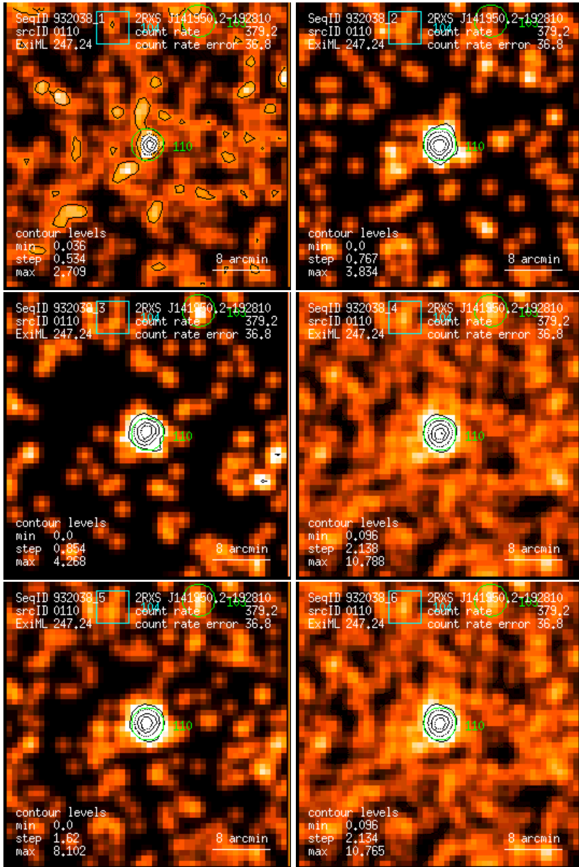
Figure 110: RASS 932038: detection 0110: band rate images, Gaussian filter: (1) PSPC channels 11 – 41, (2) 52 – 90, (3) 91 – 201, (4) 11 – 235, (5) 52 – 201, (6) 11 – 201. Broad band rates in counts/ks. Band rate contour levels in counts/ks/arcmin 2 .
