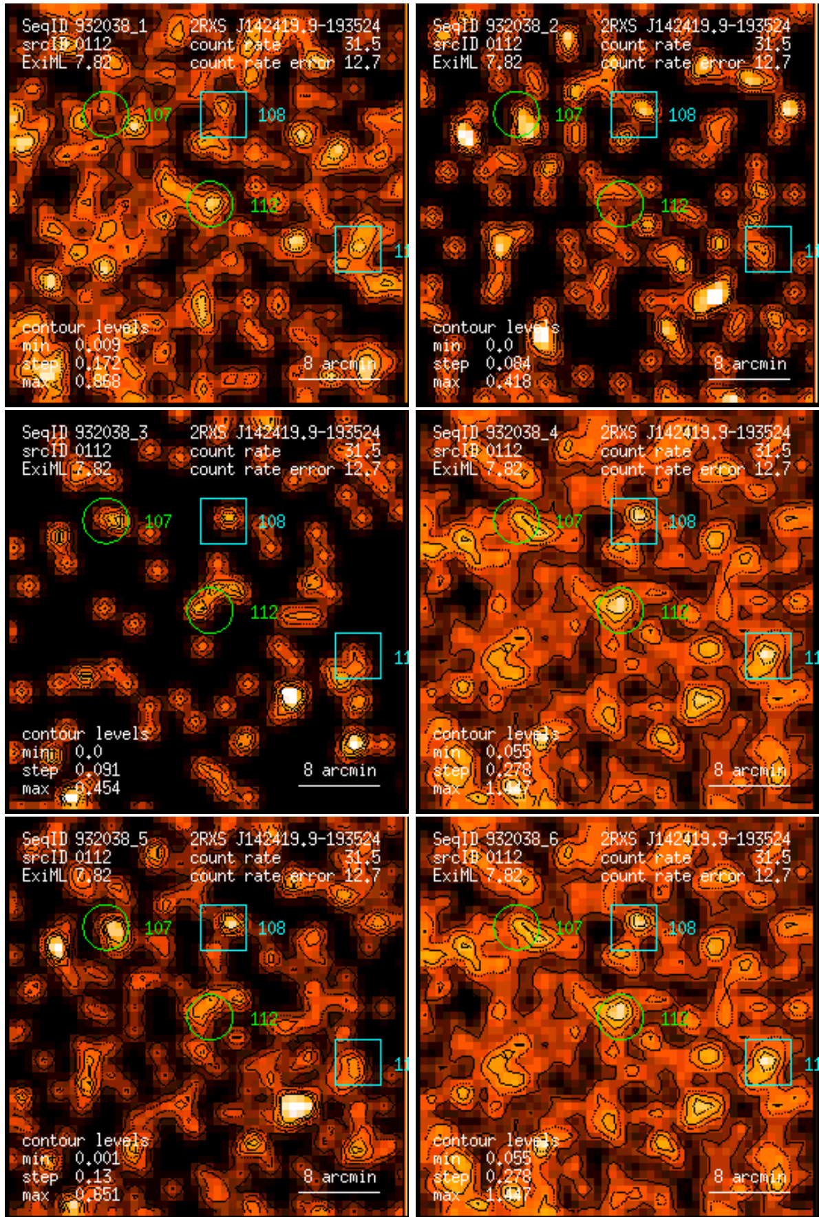
Figure 112: RASS 932038: detection 0112: band rate images, Gaussian filter: (1) PSPC channels 11 – 41, (2) 52 – 90, (3) 91 – 201, (4) 11 – 235, (5) 52 – 201, (6) 11 – 201. Broad band rates in counts/ks. Band rate contour levels in counts/ks/arcmin 2 .
