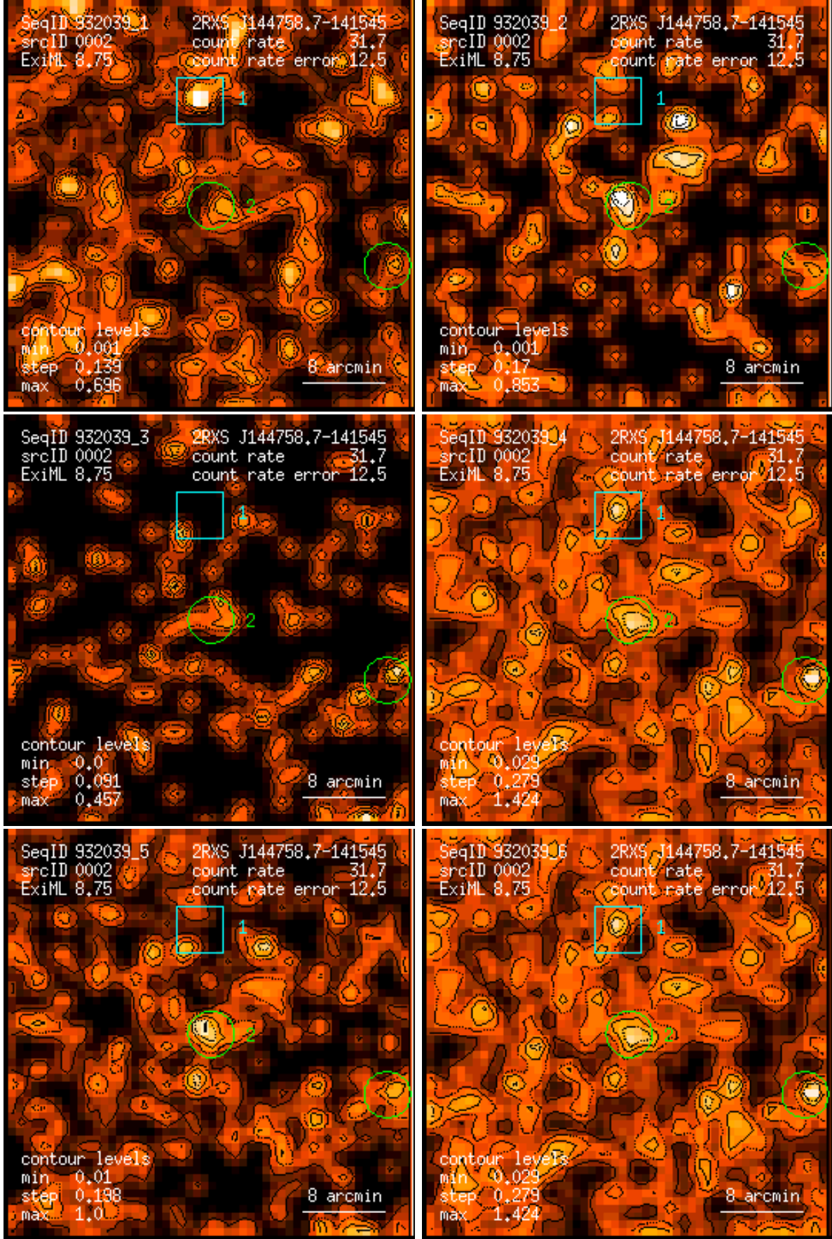
Figure 2: RASS 932039: detection 0002: band rate images, Gaussian filter: (1) PSPC channels 11 – 41, (2) 52 – 90, (3) 91 – 201, (4) 11 – 235, (5) 52 – 201, (6) 11 – 201. Broad band rates in counts/ks. Band rate contour levels in counts/ks/arcmin 2 .
