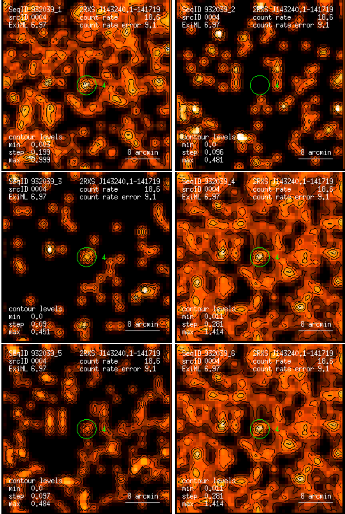
Figure 4: RASS 932039: detection 0004: band rate images, Gaussian filter: (1) PSPC channels 11 – 41, (2) 52 – 90, (3) 91 – 201, (4) 11 – 235, (5) 52 – 201, (6) 11 – 201. Broad band rates in counts/ks. Band rate contour levels in counts/ks/arcmin 2 .
