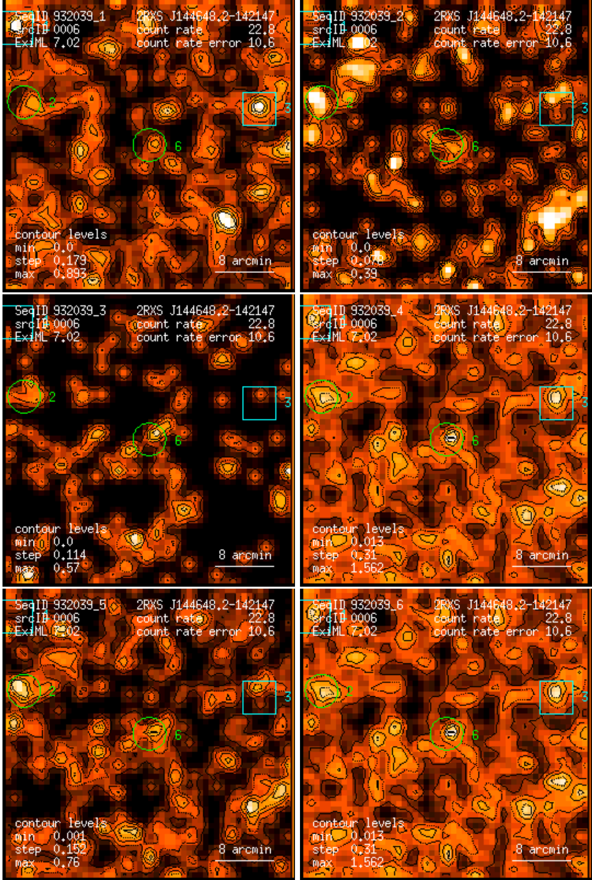
Figure 6: RASS 932039: detection 0006: band rate images, Gaussian filter: (1) PSPC channels 11 – 41, (2) 52 – 90, (3) 91 – 201, (4) 11 – 235, (5) 52 – 201, (6) 11 – 201. Broad band rates in counts/ks. Band rate contour levels in counts/ks/arcmin 2 .
