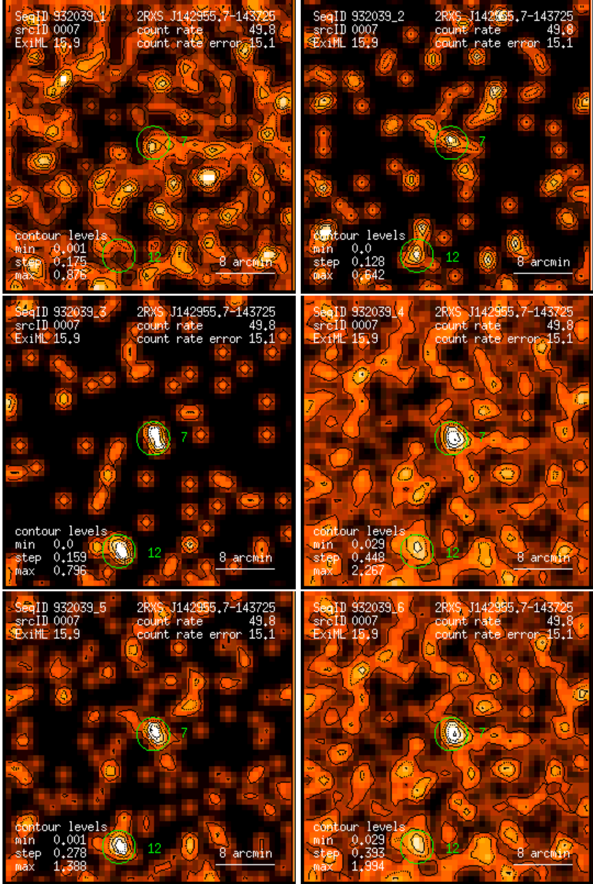
Figure 7: RASS 932039: detection 0007: band rate images, Gaussian filter: (1) PSPC channels 11 – 41, (2) 52 – 90, (3) 91 – 201, (4) 11 – 235, (5) 52 – 201, (6) 11 – 201. Broad band rates in counts/ks. Band rate contour levels in counts/ks/arcmin 2 .
