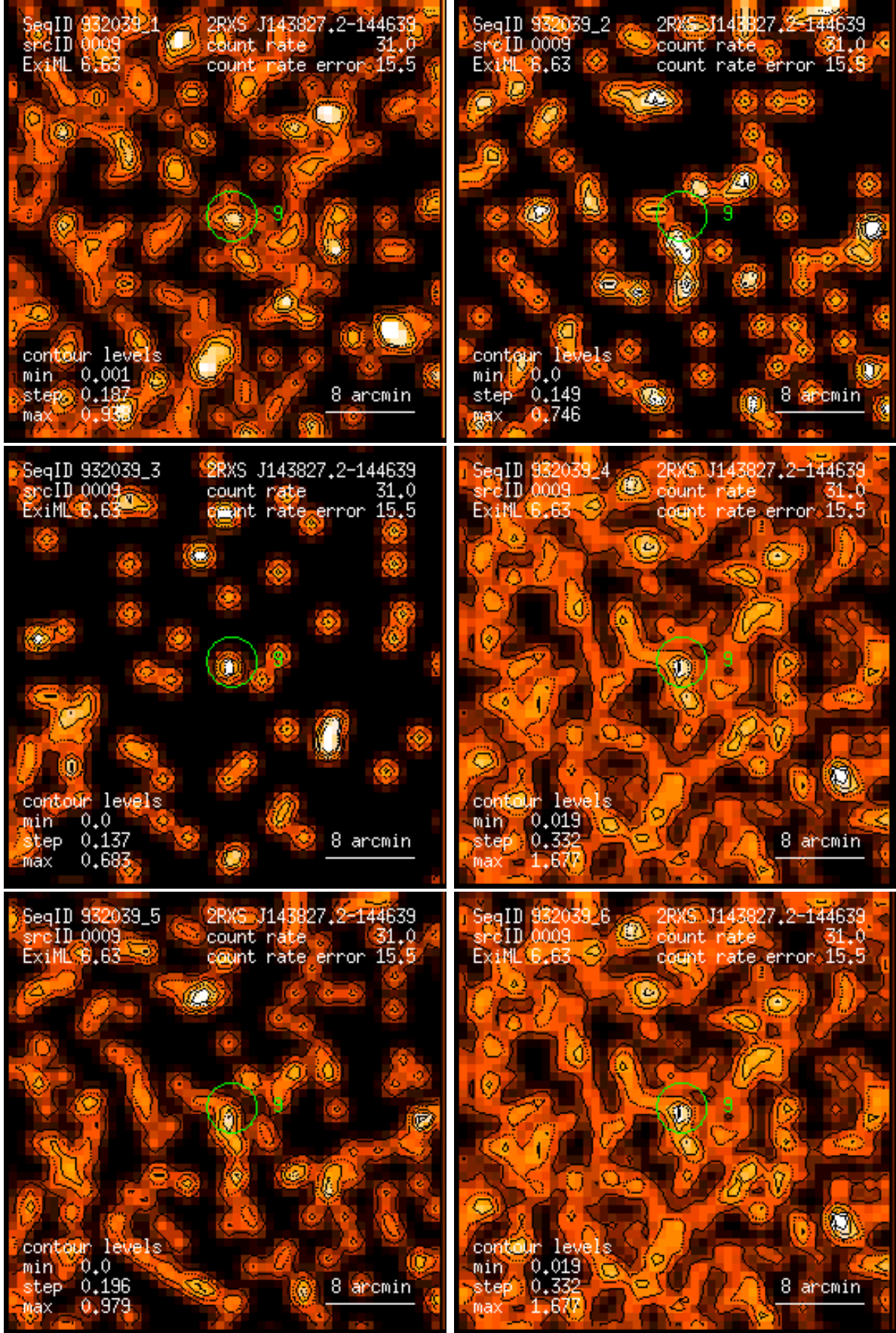
Figure 9: RASS 932039: detection 0009: band rate images, Gaussian filter: (1) PSPC channels 11 – 41, (2) 52 – 90, (3) 91 – 201, (4) 11 – 235, (5) 52 – 201, (6) 11 – 201. Broad band rates in counts/ks. Band rate contour levels in counts/ks/arcmin 2 .
