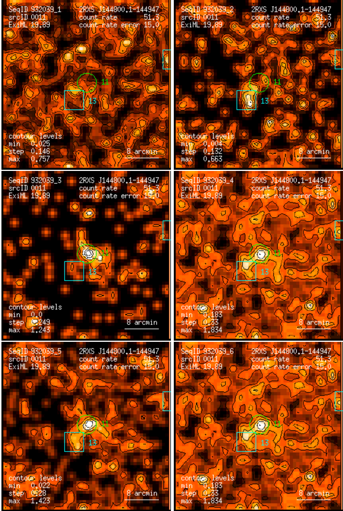
Figure 11: RASS 932039: detection 0011: band rate images, Gaussian filter: (1) PSPC channels 11 – 41, (2) 52 – 90, (3) 91 – 201, (4) 11 – 235, (5) 52 – 201, (6) 11 – 201. Broad band rates in counts/ks. Band rate contour levels in counts/ks/arcmin 2 .
