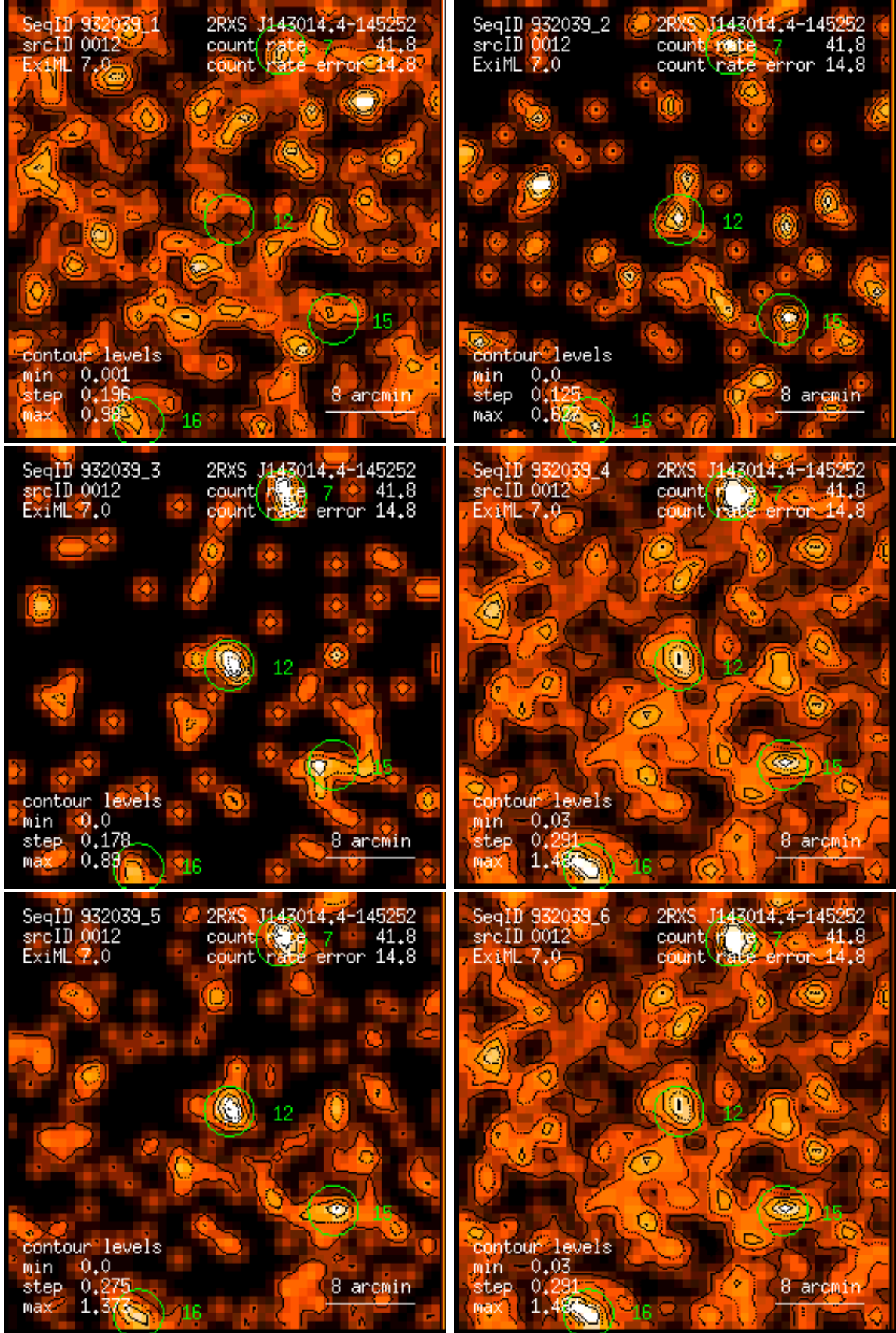
Figure 12: RASS 932039: detection 0012: band rate images, Gaussian filter: (1) PSPC channels 11 – 41, (2) 52 – 90, (3) 91 – 201, (4) 11 – 235, (5) 52 – 201, (6) 11 – 201. Broad band rates in counts/ks. Band rate contour levels in counts/ks/arcmin 2 .
