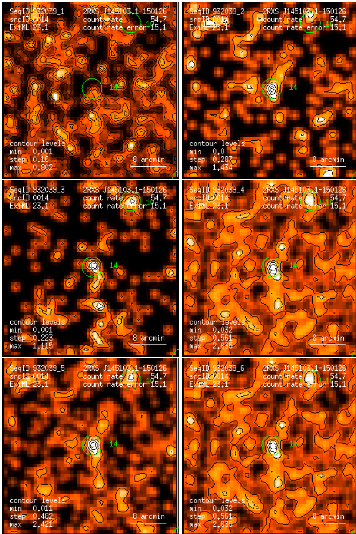
Figure 14: RASS 932039: detection 0014: band rate images, Gaussian filter: (1) PSPC channels 11 – 41, (2) 52 – 90, (3) 91 – 201, (4) 11 – 235, (5) 52 – 201, (6) 11 – 201. Broad band rates in counts/ks. Band rate contour levels in counts/ks/arcmin 2 .
