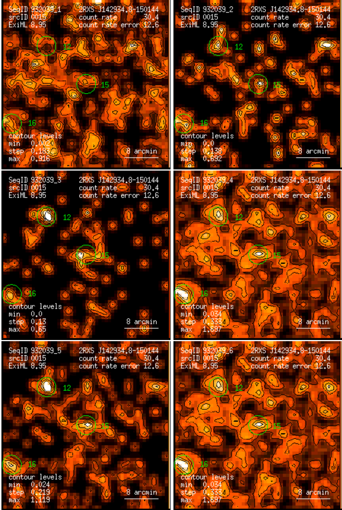
Figure 15: RASS 932039: detection 0015: band rate images, Gaussian filter: (1) PSPC channels 11 – 41, (2) 52 – 90, (3) 91 – 201, (4) 11 – 235, (5) 52 – 201, (6) 11 – 201. Broad band rates in counts/ks. Band rate contour levels in counts/ks/arcmin 2 .
