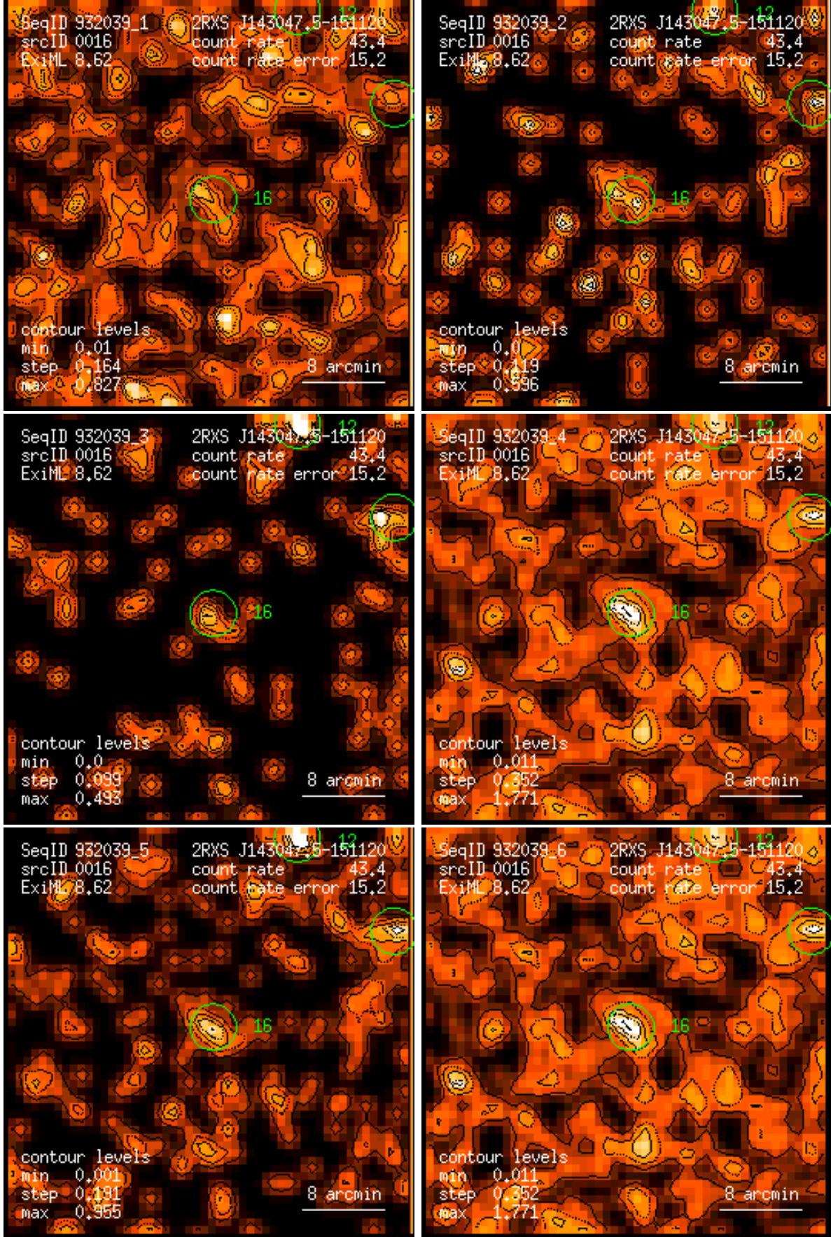
Figure 16: RASS 932039: detection 0016: band rate images, Gaussian filter: (1) PSPC channels 11 – 41, (2) 52 – 90, (3) 91 – 201, (4) 11 – 235, (5) 52 – 201, (6) 11 – 201. Broad band rates in counts/ks. Band rate contour levels in counts/ks/arcmin 2 .
