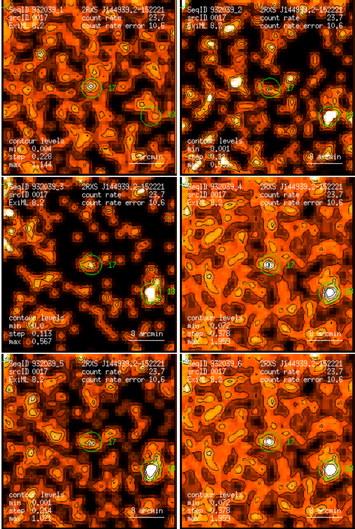
Figure 17: RASS 932039: detection 0017: band rate images, Gaussian filter: (1) PSPC channels 11 – 41, (2) 52 – 90, (3) 91 – 201, (4) 11 – 235, (5) 52 – 201, (6) 11 – 201. Broad band rates in counts/ks. Band rate contour levels in counts/ks/arcmin 2 .
