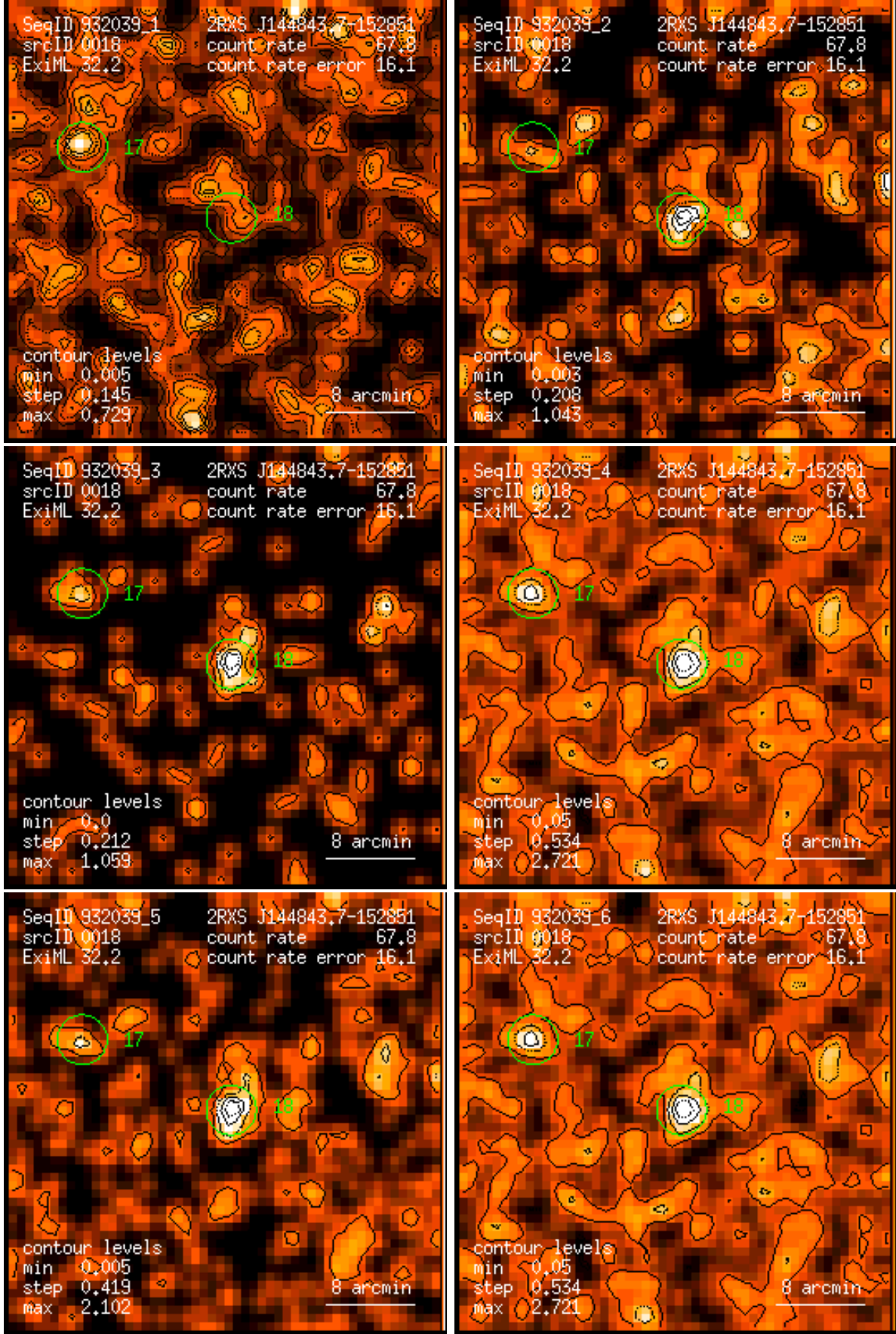
Figure 18: RASS 932039: detection 0018: band rate images, Gaussian filter: (1) PSPC channels 11 – 41, (2) 52 – 90, (3) 91 – 201, (4) 11 – 235, (5) 52 – 201, (6) 11 – 201. Broad band rates in counts/ks. Band rate contour levels in counts/ks/arcmin 2 .
