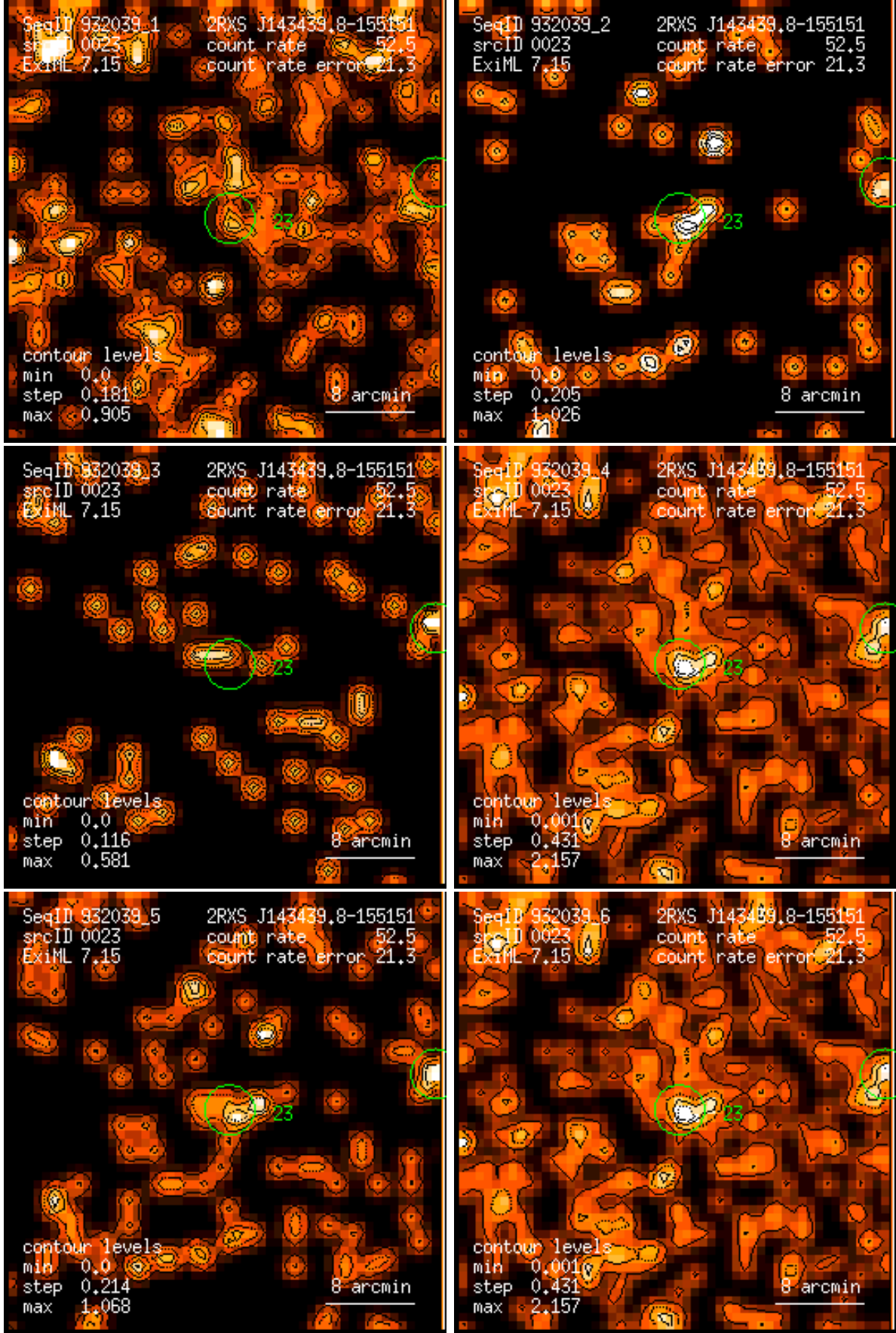
Figure 23: RASS 932039: detection 0023: band rate images, Gaussian filter: (1) PSPC channels 11 – 41, (2) 52 – 90, (3) 91 – 201, (4) 11 – 235, (5) 52 – 201, (6) 11 – 201. Broad band rates in counts/ks. Band rate contour levels in counts/ks/arcmin 2 .
