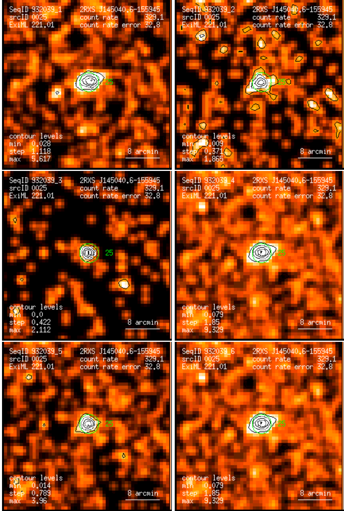
Figure 25: RASS 932039: detection 0025: band rate images, Gaussian filter: (1) PSPC channels 11 – 41, (2) 52 – 90, (3) 91 – 201, (4) 11 – 235, (5) 52 – 201, (6) 11 – 201. Broad band rates in counts/ks. Band rate contour levels in counts/ks/arcmin 2 .
