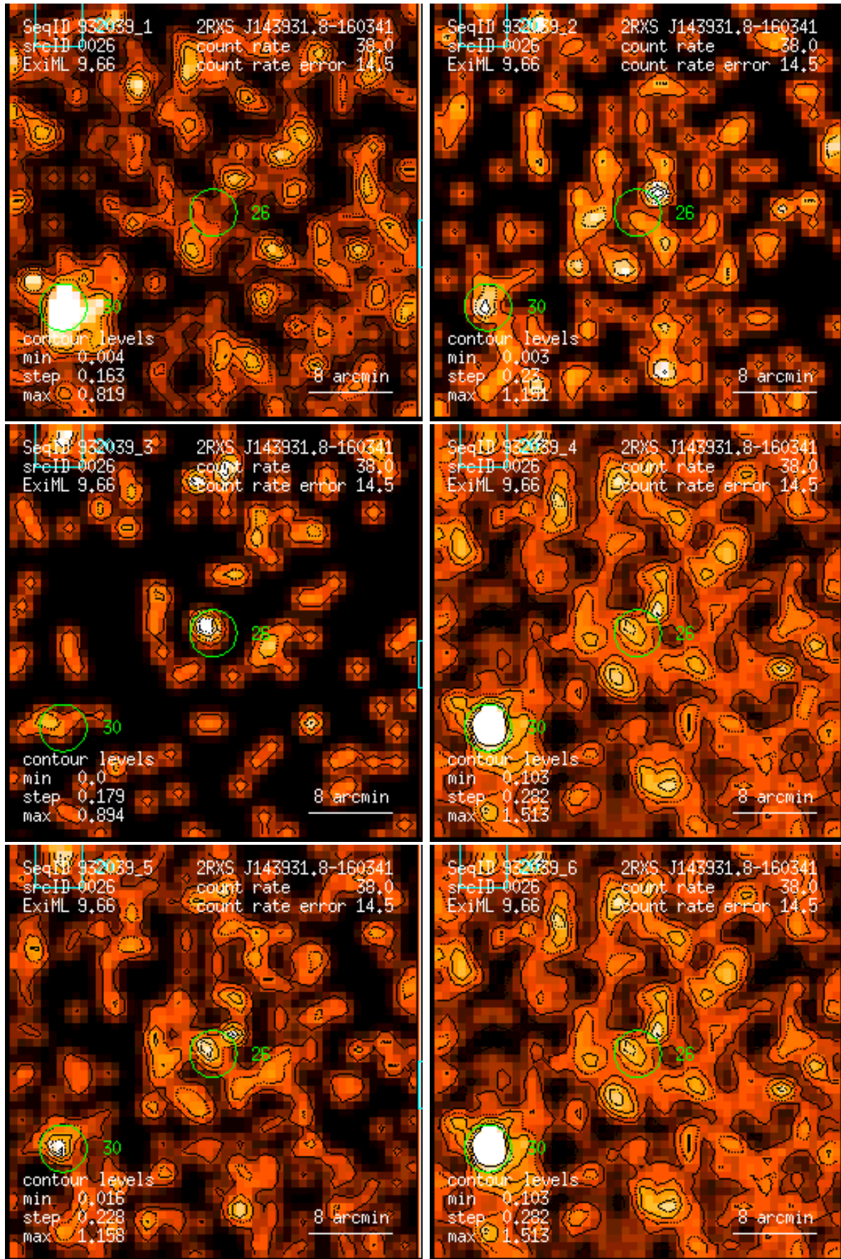
Figure 26: RASS 932039: detection 0026: band rate images, Gaussian filter: (1) PSPC channels 11 – 41, (2) 52 – 90, (3) 91 – 201, (4) 11 – 235, (5) 52 – 201, (6) 11 – 201. Broad band rates in counts/ks. Band rate contour levels in counts/ks/arcmin 2 .
