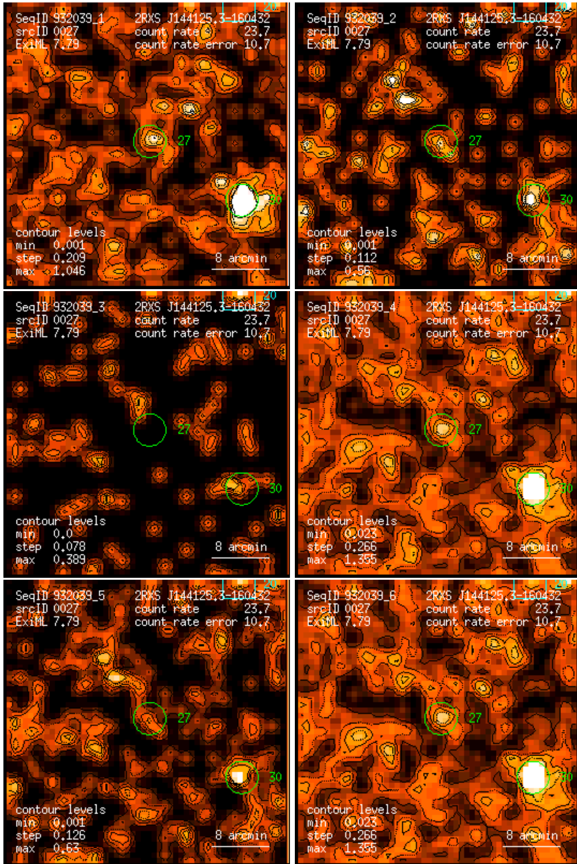
Figure 27: RASS 932039: detection 0027: band rate images, Gaussian filter: (1) PSPC channels 11 – 41, (2) 52 – 90, (3) 91 – 201, (4) 11 – 235, (5) 52 – 201, (6) 11 – 201. Broad band rates in counts/ks. Band rate contour levels in counts/ks/arcmin 2 .
