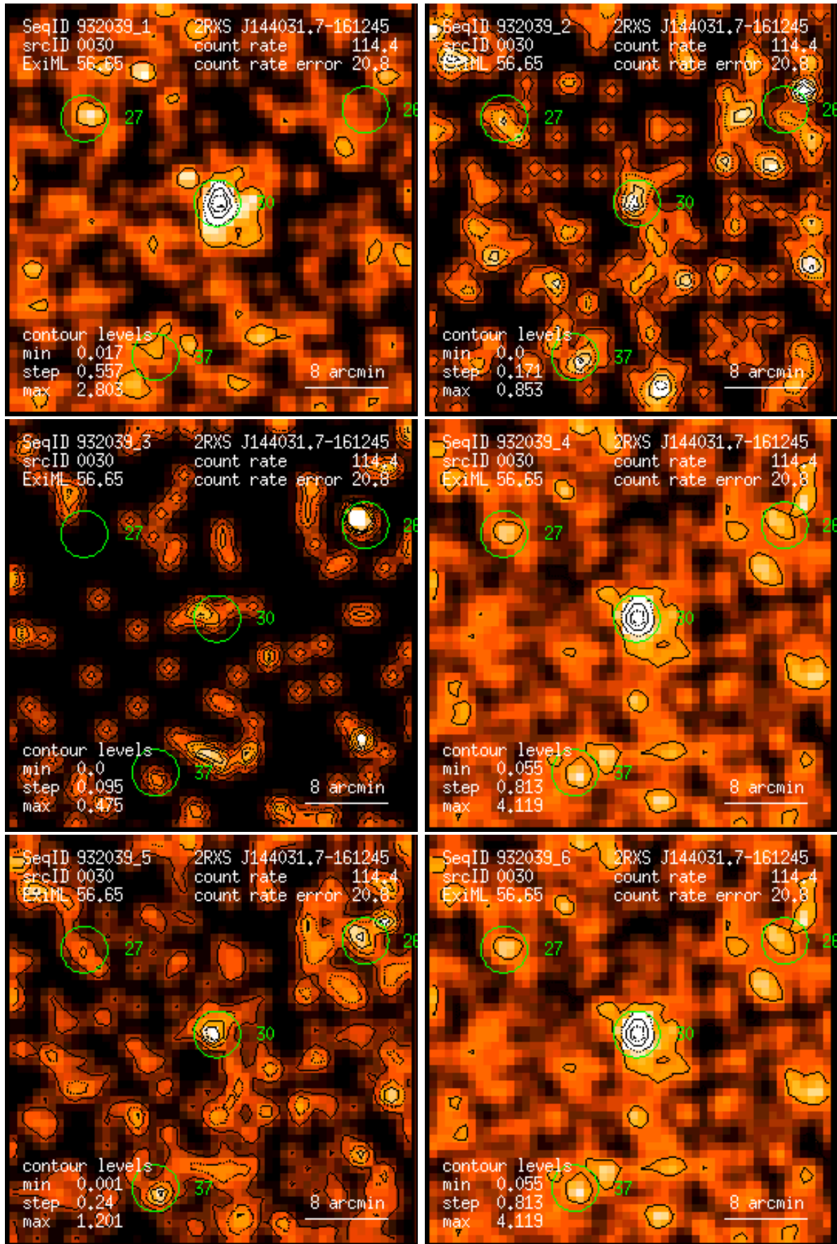
Figure 30: RASS 932039: detection 0030: band rate images, Gaussian filter: (1) PSPC channels 11 – 41, (2) 52 – 90, (3) 91 – 201, (4) 11 – 235, (5) 52 – 201, (6) 11 – 201. Broad band rates in counts/ks. Band rate contour levels in counts/ks/arcmin 2 .
