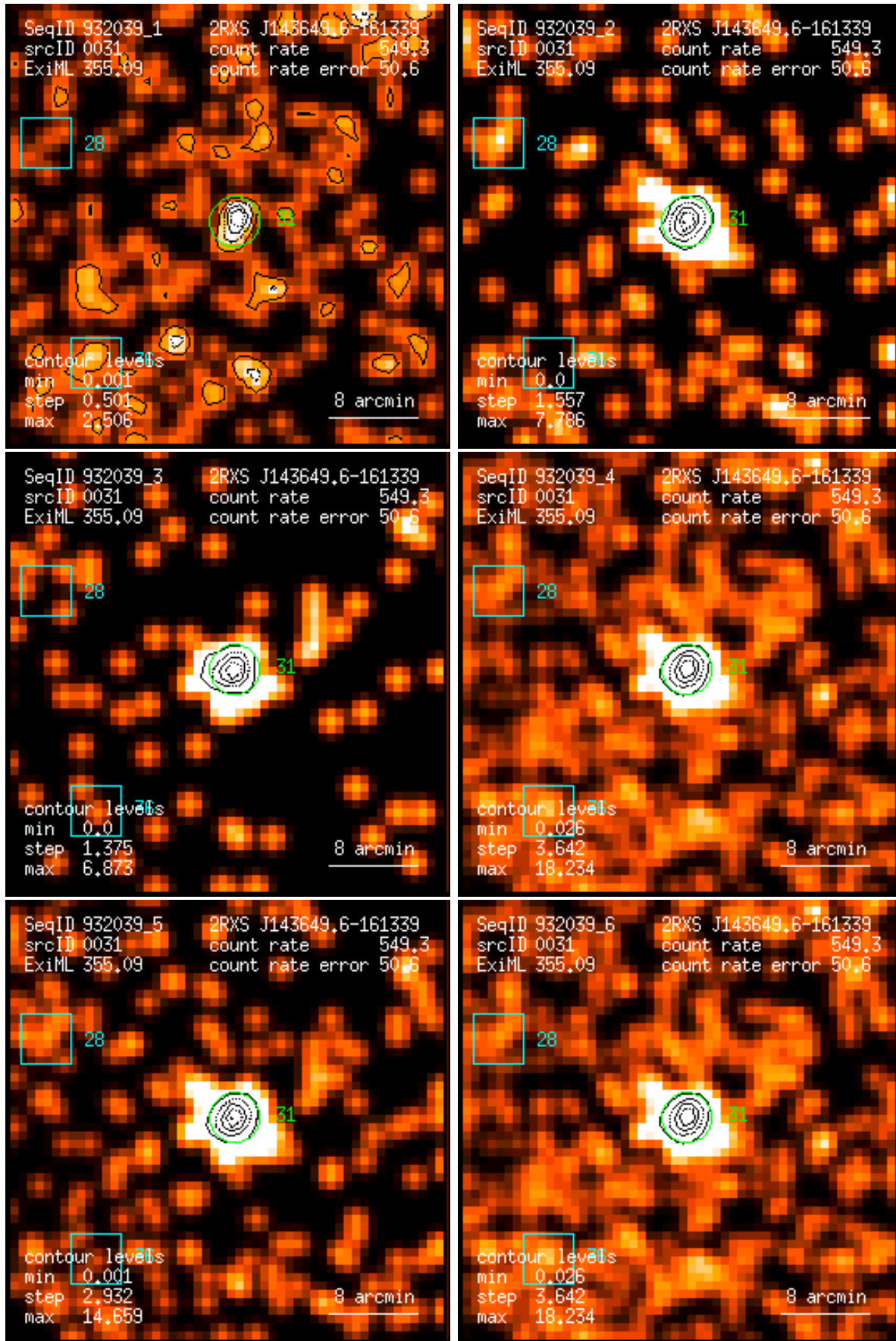
Figure 31: RASS 932039: detection 0031: band rate images, Gaussian filter: (1) PSPC channels 11 – 41, (2) 52 – 90, (3) 91 – 201, (4) 11 – 235, (5) 52 – 201, (6) 11 – 201. Broad band rates in counts/ks. Band rate contour levels in counts/ks/arcmin 2 .
