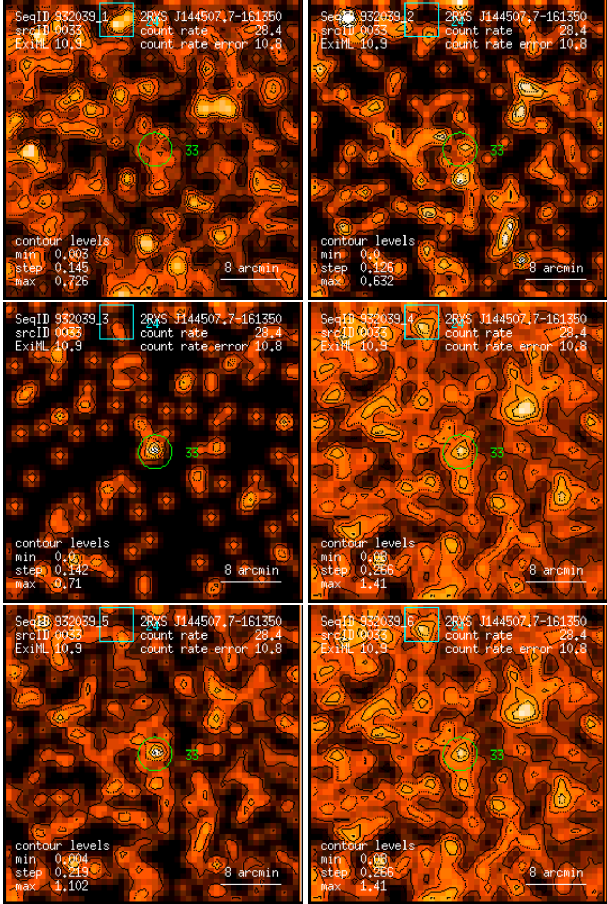
Figure 33: RASS 932039: detection 0033: band rate images, Gaussian filter: (1) PSPC channels 11 – 41, (2) 52 – 90, (3) 91 – 201, (4) 11 – 235, (5) 52 – 201, (6) 11 – 201. Broad band rates in counts/ks. Band rate contour levels in counts/ks/arcmin 2 .
