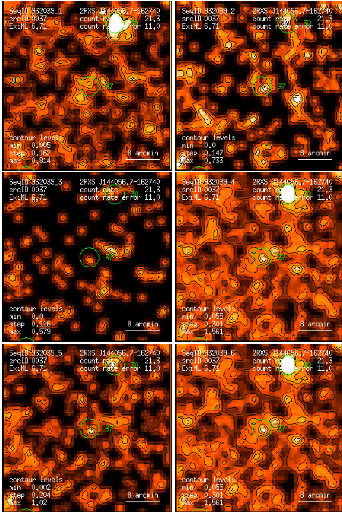
Figure 37: RASS 932039: detection 0037: band rate images, Gaussian filter: (1) PSPC channels 11 – 41, (2) 52 – 90, (3) 91 – 201, (4) 11 – 235, (5) 52 – 201, (6) 11 – 201. Broad band rates in counts/ks. Band rate contour levels in counts/ks/arcmin 2 .
