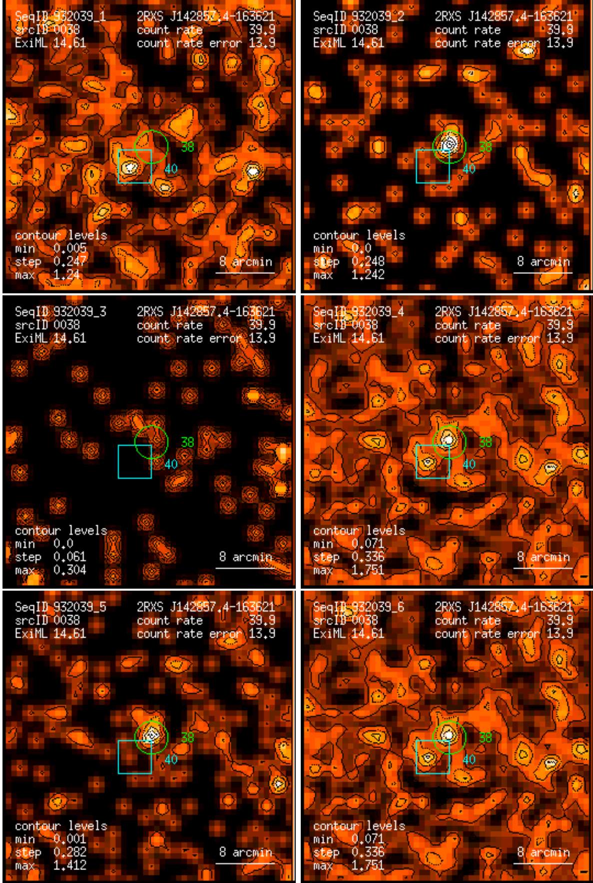
Figure 38: RASS 932039: detection 0038: band rate images, Gaussian filter: (1) PSPC channels 11 – 41, (2) 52 – 90, (3) 91 – 201, (4) 11 – 235, (5) 52 – 201, (6) 11 – 201. Broad band rates in counts/ks. Band rate contour levels in counts/ks/arcmin 2 .
