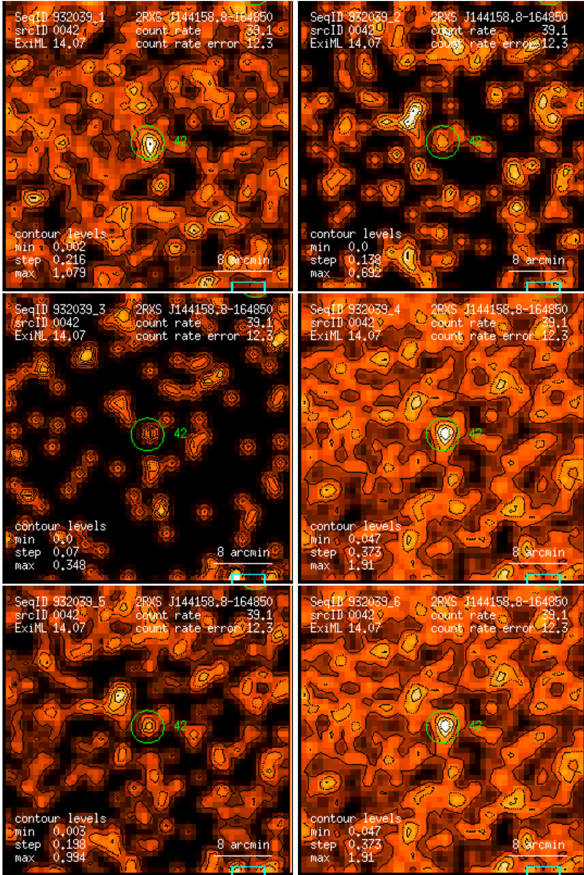
Figure 42: RASS 932039: detection 0042: band rate images, Gaussian filter: (1) PSPC channels 11 – 41, (2) 52 – 90, (3) 91 – 201, (4) 11 – 235, (5) 52 – 201, (6) 11 – 201. Broad band rates in counts/ks. Band rate contour levels in counts/ks/arcmin 2 .
