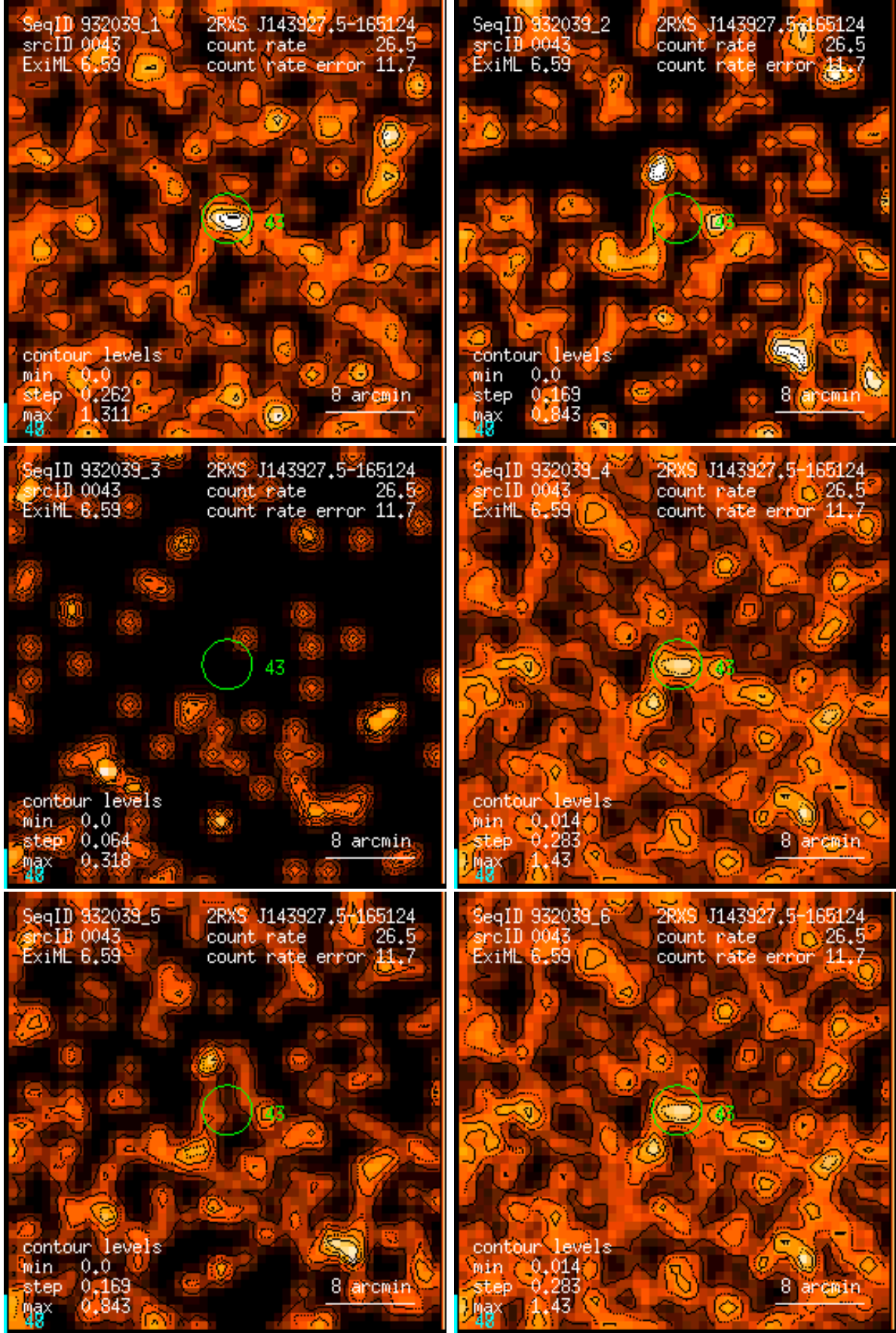
Figure 43: RASS 932039: detection 0043: band rate images, Gaussian filter: (1) PSPC channels 11 – 41, (2) 52 – 90, (3) 91 – 201, (4) 11 – 235, (5) 52 – 201, (6) 11 – 201. Broad band rates in counts/ks. Band rate contour levels in counts/ks/arcmin 2 .
