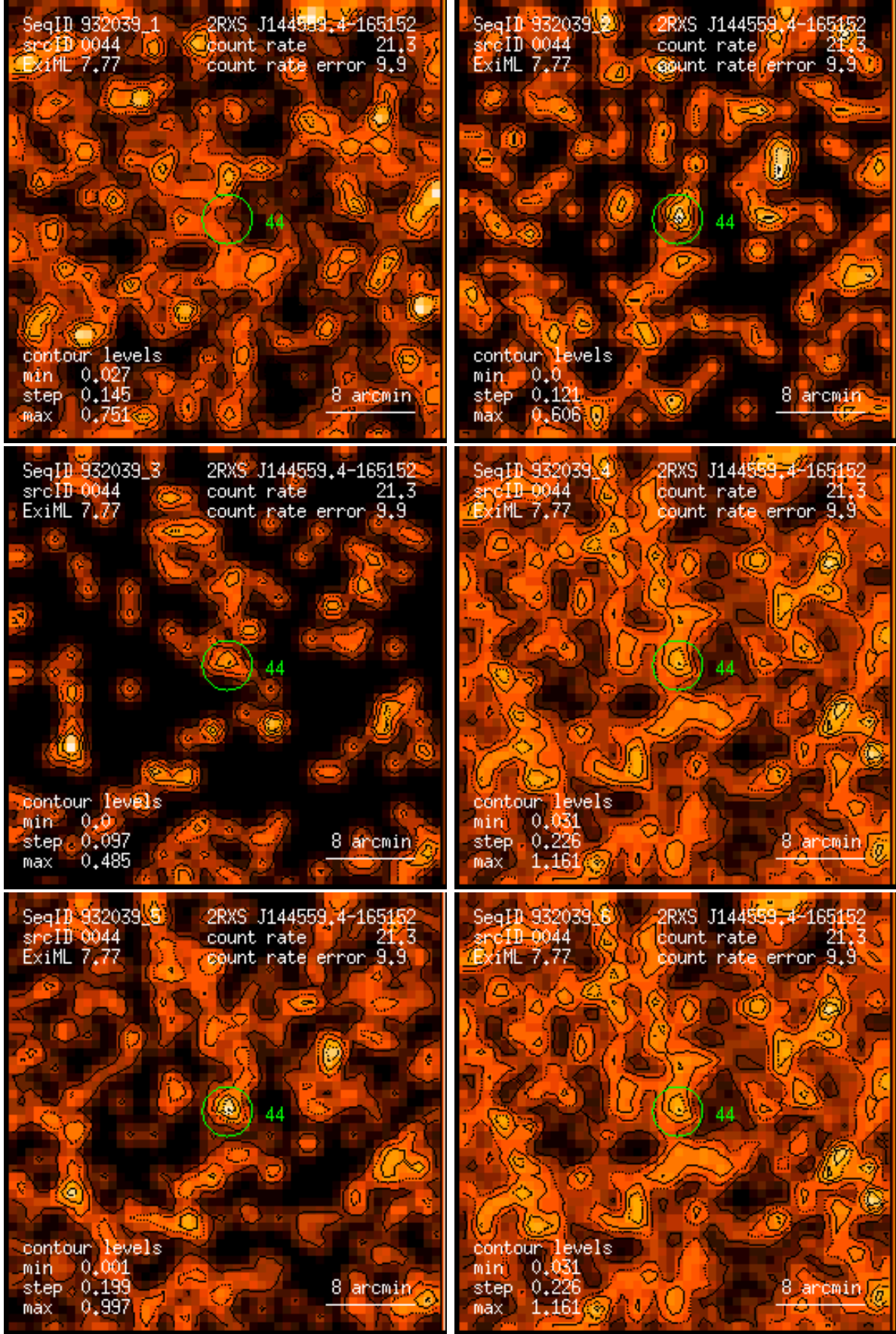
Figure 44: RASS 932039: detection 0044: band rate images, Gaussian filter: (1) PSPC channels 11 – 41, (2) 52 – 90, (3) 91 – 201, (4) 11 – 235, (5) 52 – 201, (6) 11 – 201. Broad band rates in counts/ks. Band rate contour levels in counts/ks/arcmin 2 .
