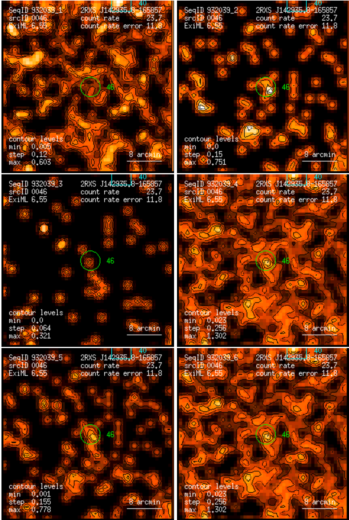
Figure 46: RASS 932039: detection 0046: band rate images, Gaussian filter: (1) PSPC channels 11 – 41, (2) 52 – 90, (3) 91 – 201, (4) 11 – 235, (5) 52 – 201, (6) 11 – 201. Broad band rates in counts/ks. Band rate contour levels in counts/ks/arcmin 2 .
