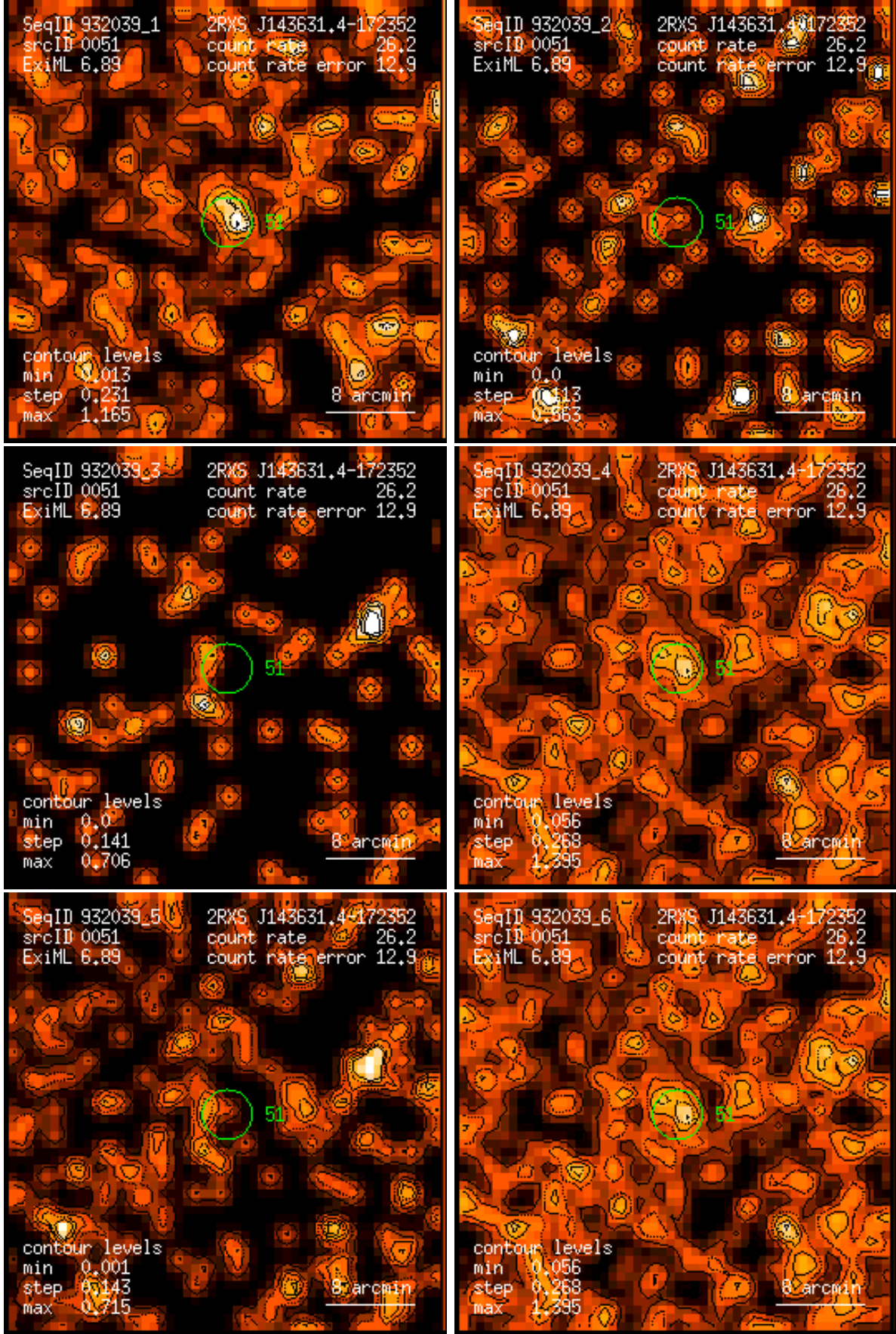
Figure 51: RASS 932039: detection 0051: band rate images, Gaussian filter: (1) PSPC channels 11 – 41, (2) 52 – 90, (3) 91 – 201, (4) 11 – 235, (5) 52 – 201, (6) 11 – 201. Broad band rates in counts/ks. Band rate contour levels in counts/ks/arcmin 2 .
