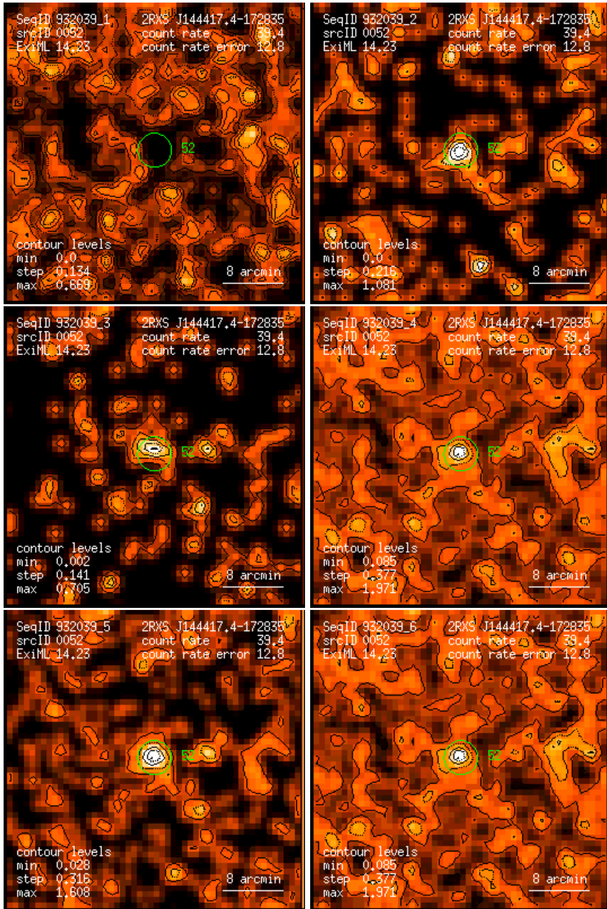
Figure 52: RASS 932039: detection 0052: band rate images, Gaussian filter: (1) PSPC channels 11 – 41, (2) 52 – 90, (3) 91 – 201, (4) 11 – 235, (5) 52 – 201, (6) 11 – 201. Broad band rates in counts/ks. Band rate contour levels in counts/ks/arcmin 2 .
