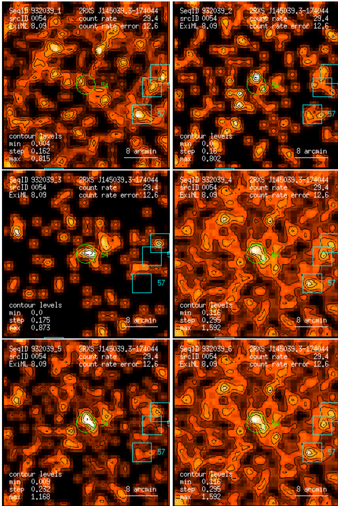
Figure 54: RASS 932039: detection 0054: band rate images, Gaussian filter: (1) PSPC channels 11 – 41, (2) 52 – 90, (3) 91 – 201, (4) 11 – 235, (5) 52 – 201, (6) 11 – 201. Broad band rates in counts/ks. Band rate contour levels in counts/ks/arcmin 2 .
